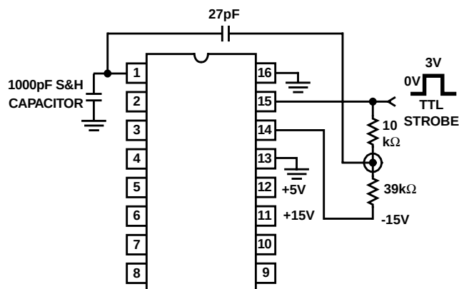
FIGURE 8. NO-ADJUST CHARGE INJECTION COMPENSATION CIRCUIT
