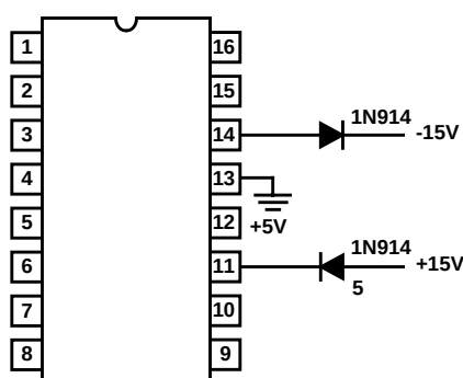
FIGURE 9. ADDING DIODES PROTECTS SWITCH
