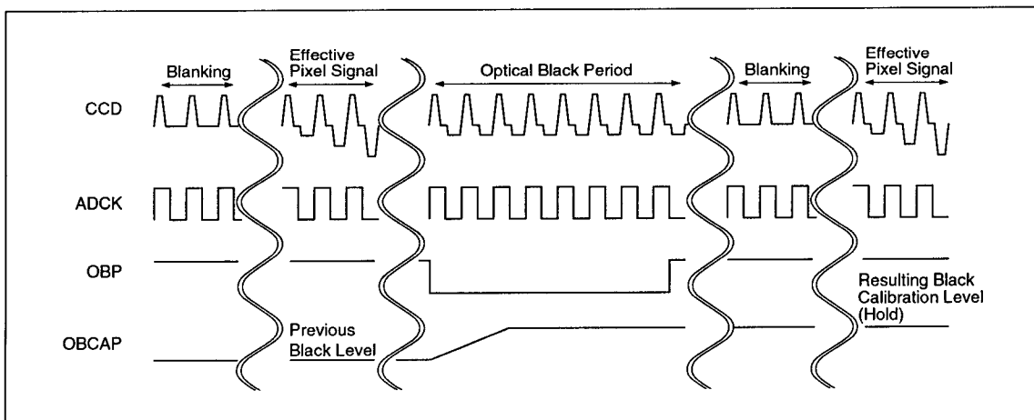
Black Level Calibration Timing
