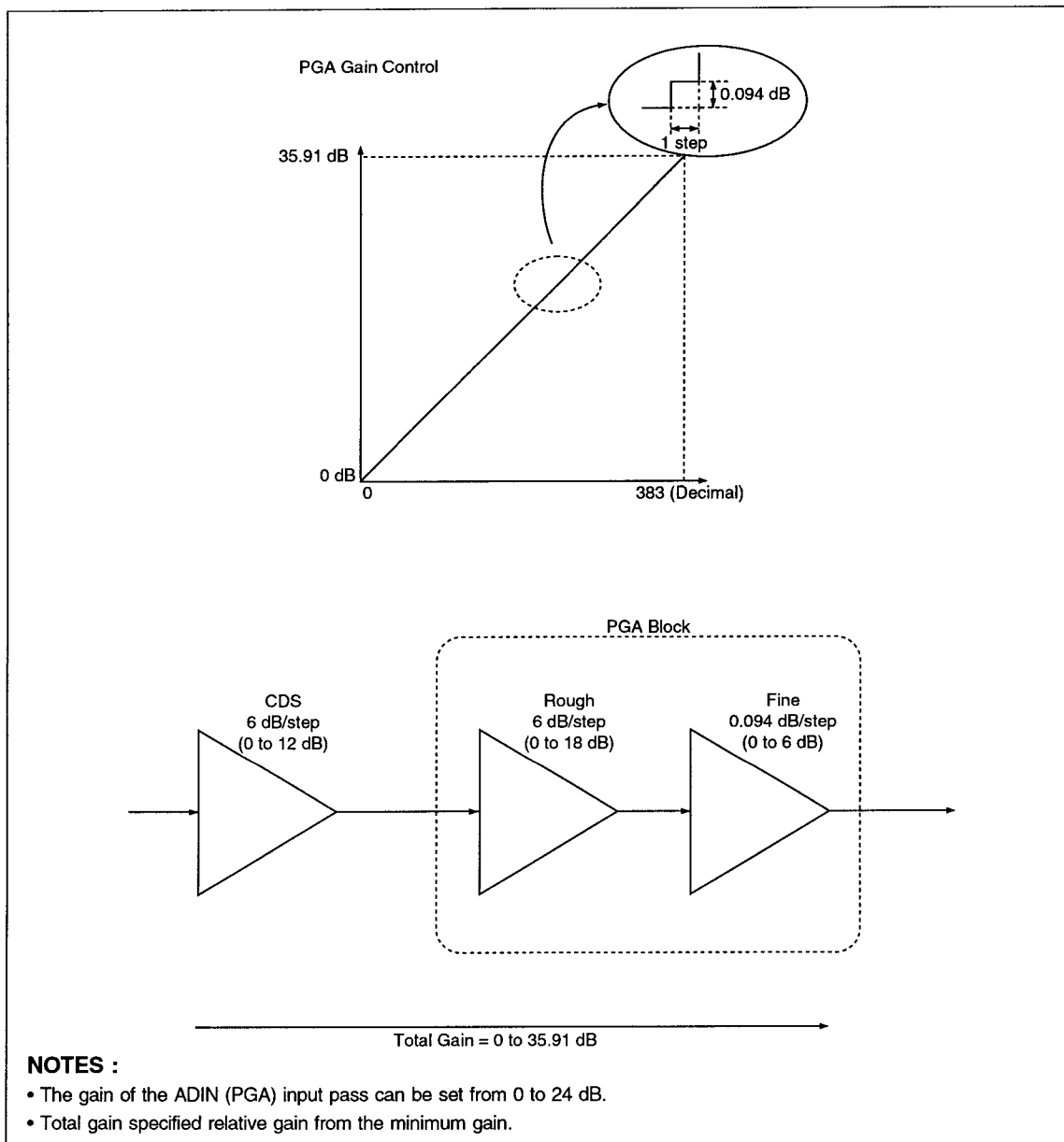
Gain Control
