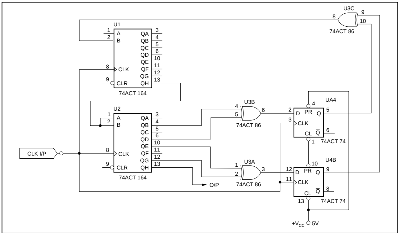
FIGURE 7. NRZ Psuedo-Noise Generator.
