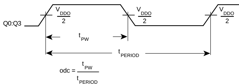
t_{PW} & t_{PERIOD}
