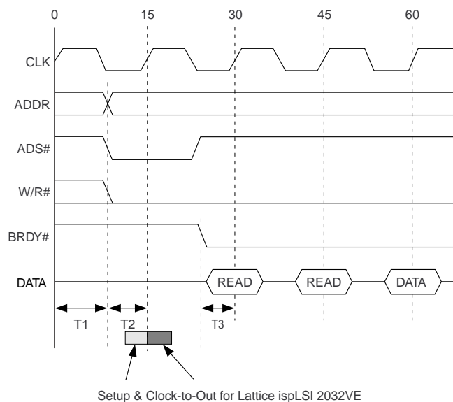
Figure 1. Pentium Burst Read-Cycle With Relative Timings
