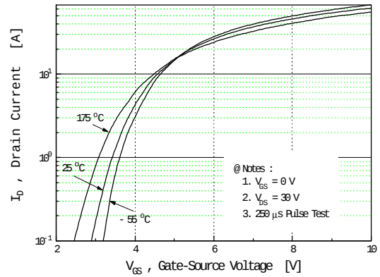
Fig 2. Transfer Characteristics
