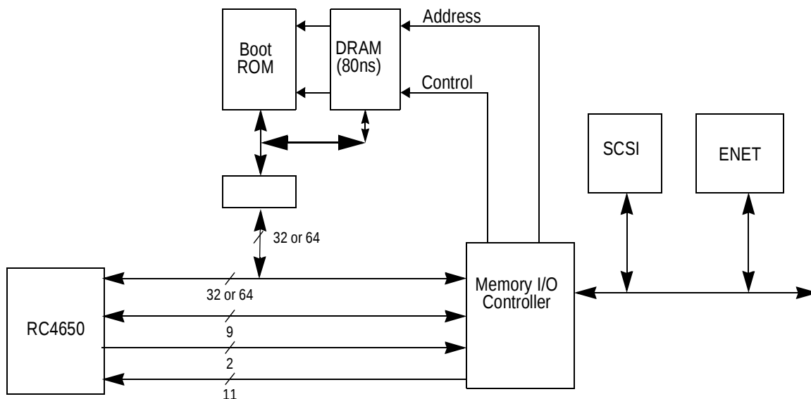
Figure 4: Typical RC4650 System Architecture
