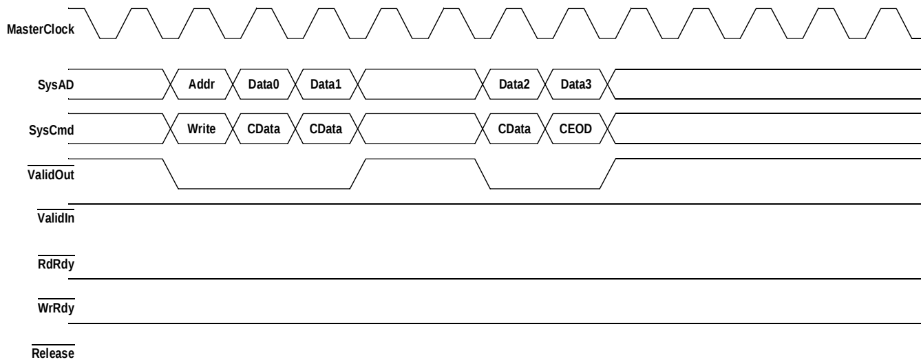
Figure 6: RC4650 Block Write Request (64-bit system interface)
