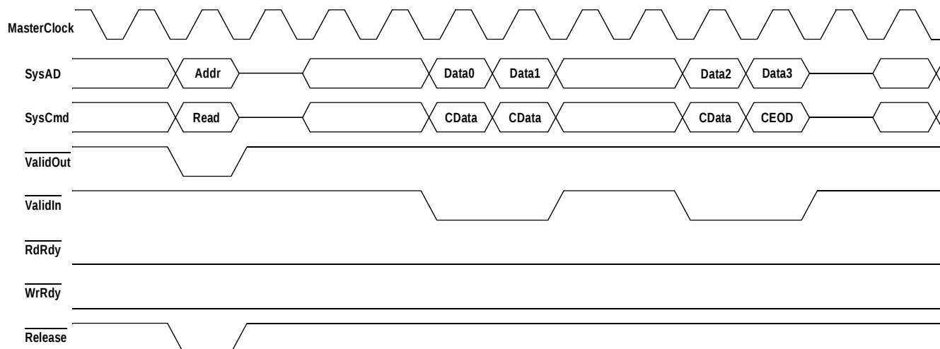
Figure 5: RC4650 Block Read Request (64-bit interface option)
