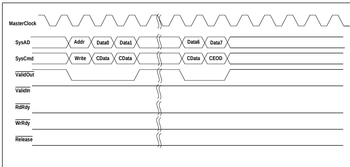
Figure 3: RC4640 Block Write Request
