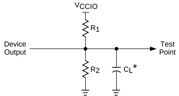
Figure 9. Test Load
