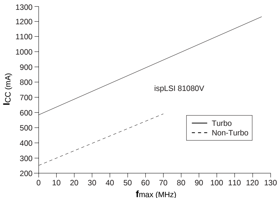
Figure 10. Typical Device Power Consumption vs fmax
