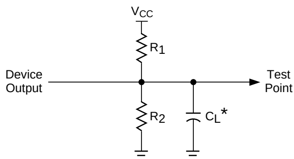
Figure 2. Test Load
