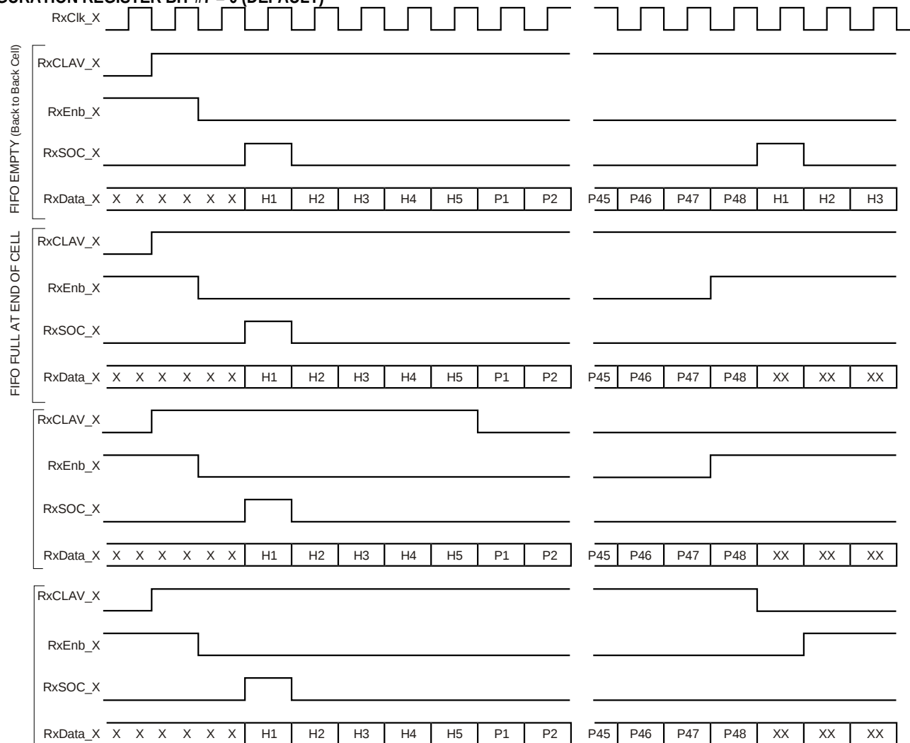
FIGURE 21. PORT A, B, C, OR D RECEIVE TIMING DIAGRAM
