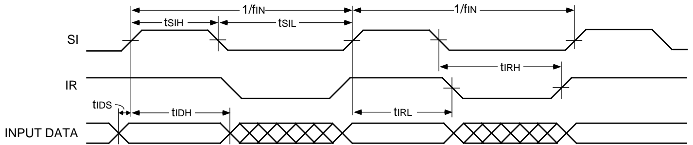
Figure 2. Input Timing
