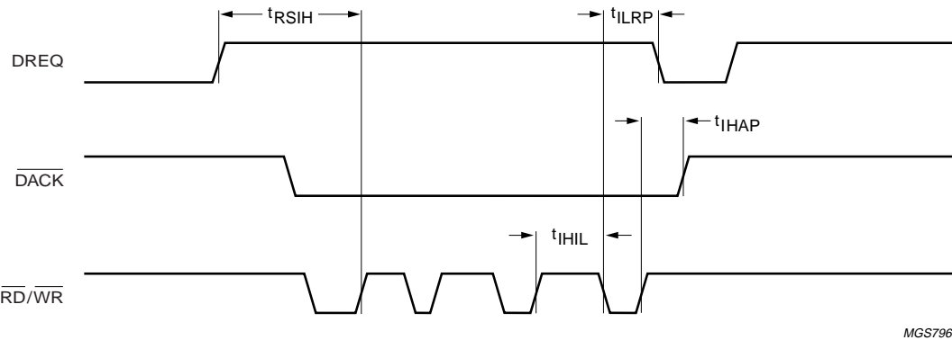
Fig 30. Burst mode DMA timing.
