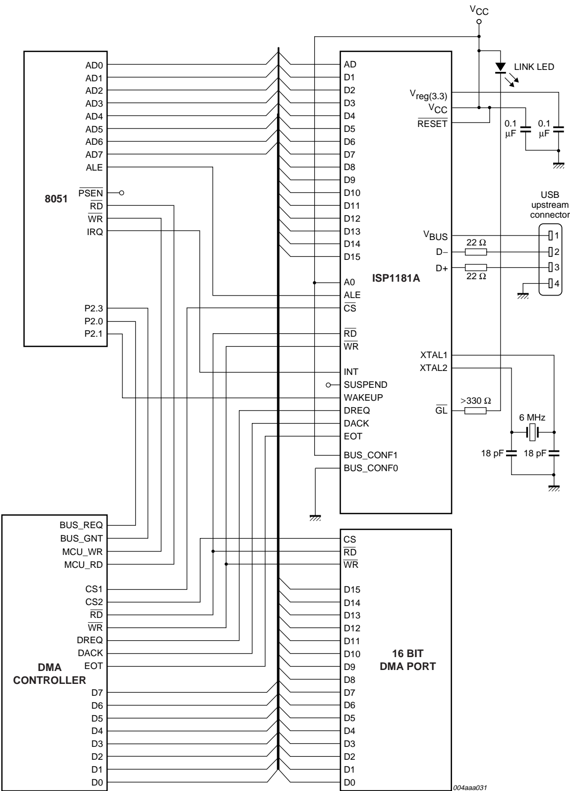
Fig 33. Typical interface circuit for bus configuration mode 2 (shared ports: 8-bit PIO, 8-bit or 16-bit DMA).
