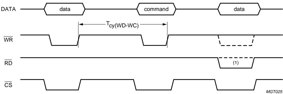
Fig 23. Write data + write command cycle timing.
