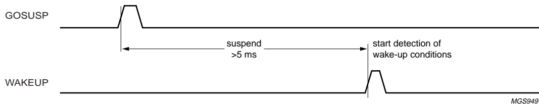
Fig 6. Typical suspend timing.
