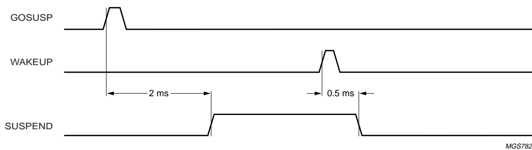
Fig 7. Suspend and resume timing for powered-off application.
