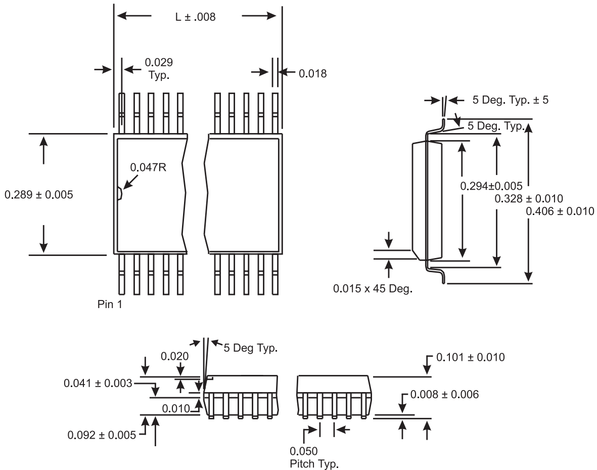
32-Pin SOIC Package
