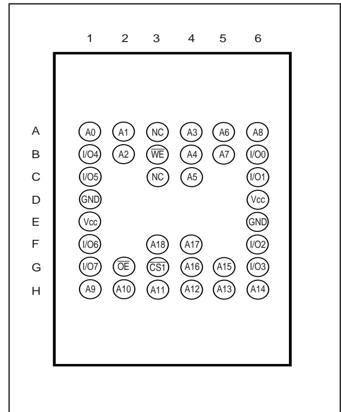
36-pin mini BGA (B) (6mm x 8mm) (Package Code B)
