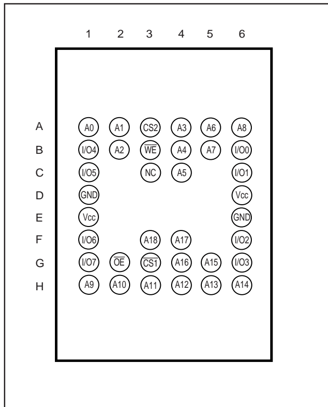
36-pin mini BGA (B) (6mm x 8mm) 2 CS Option (Package Code B2)
