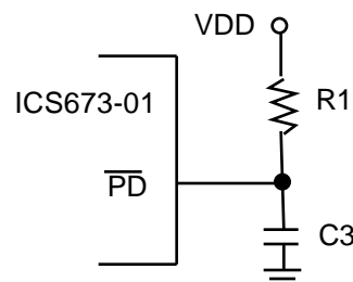
A. Basic Circuit
