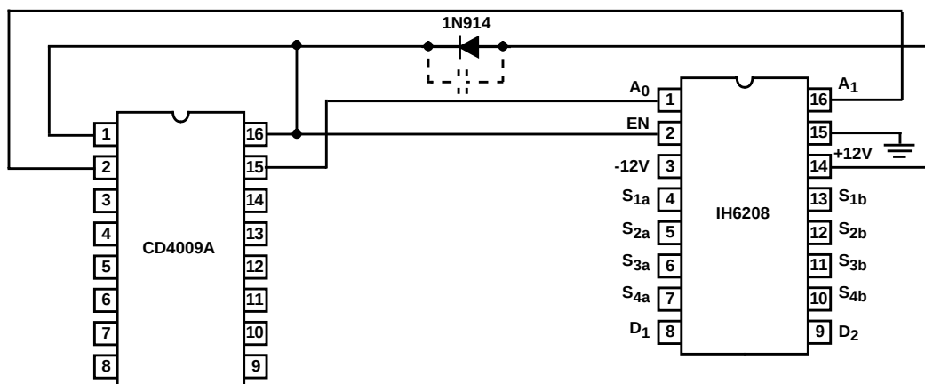
FIGURE 7. IH6208 CONNECTION DIAGRAM WITH ENABLE INPUT STROBING FOR LESS THAN \pm 15\text{V} SUPPLY OPERATION
