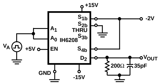
FIGURE 2. t_{\text{OPEN}} (BREAK-BEFORE-MAKE) SWITCHING TEST CIRCUIT AND WAVEFORMS
