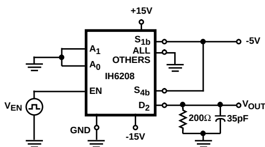
FIGURE 3. t_{\text{ON}} AND t_{\text{OFF}} SWITCHING TEST CIRCUIT AND WAVEFORMS
