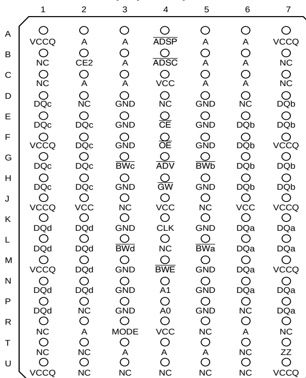
119-pin PBGA (D Version) (Top View)
