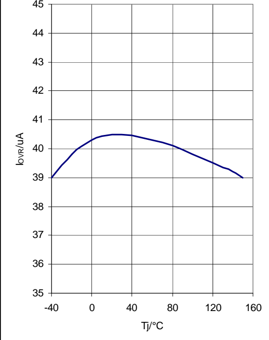
Diagram 8: I_{OVR} versus Temperature
