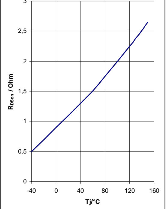
Diagram 15: R_{DSon} vs. Temperature
