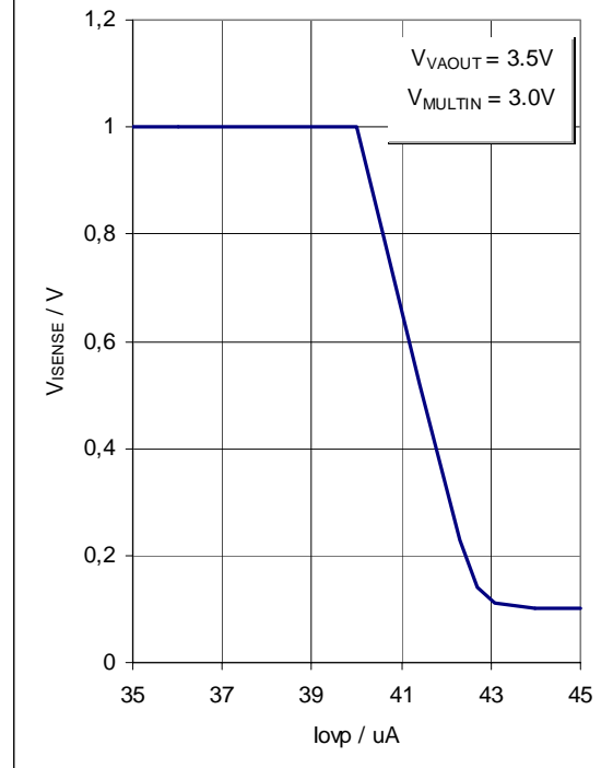
Diagram 7: Overvoltage Regulator V_{SENSE} vers. Threshold Voltage
