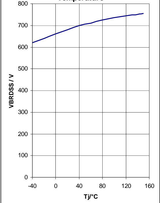
Diagram 14: V_{BRDSS} vs. Temperature
