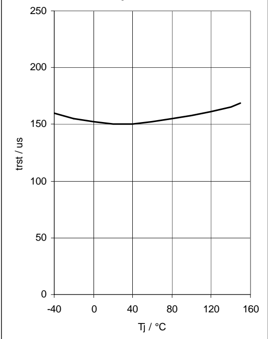
Diagram 13: Restart time versus temperature
