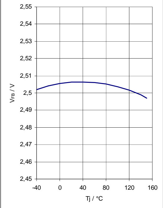
Diagram 5: V_{FB} vers. Temperature (pin1 connected to pin2)
