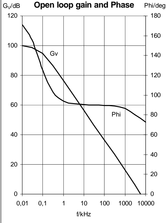
Diagram 6: Voltage Amplifier Open loop gain and Phase
