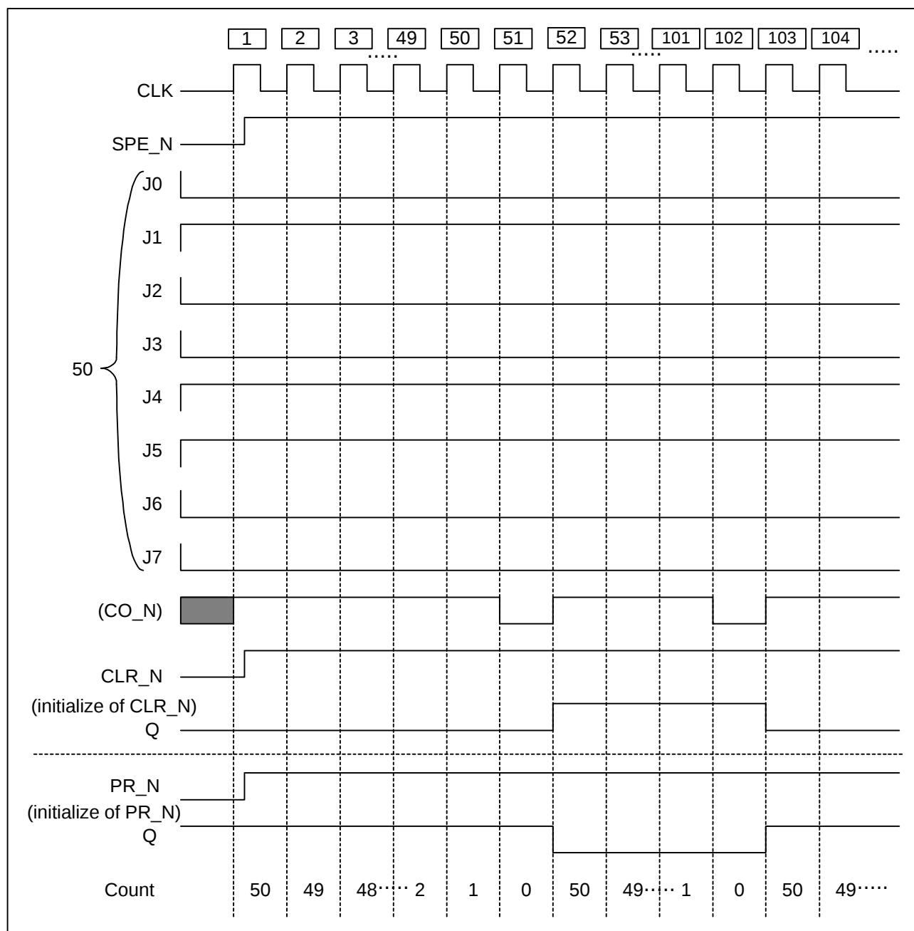
Figure 7-1. Timing Diagram When Jn is fixed
