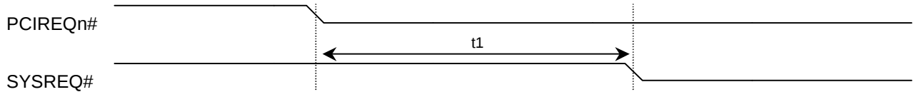
Figure 7-1. PCI Request Delay Timing
