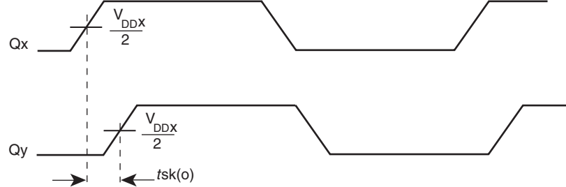
FIGURE 3 - OUTPUT SKEW
