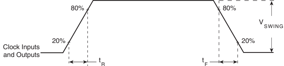
FIGURE 6 - INPUT AND OUTPUT RISE AND FALL TIME
