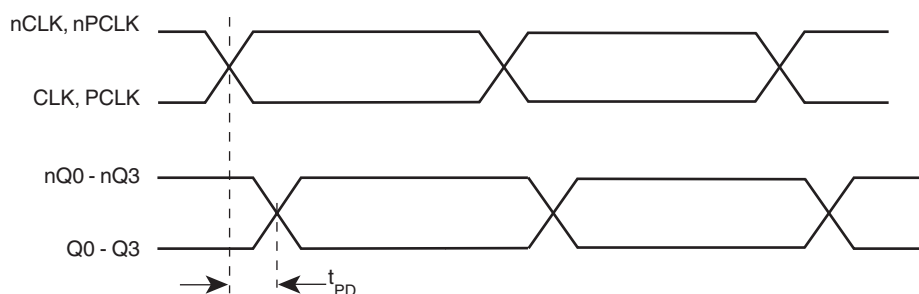
FIGURE 6 - PROPAGATION DELAY
