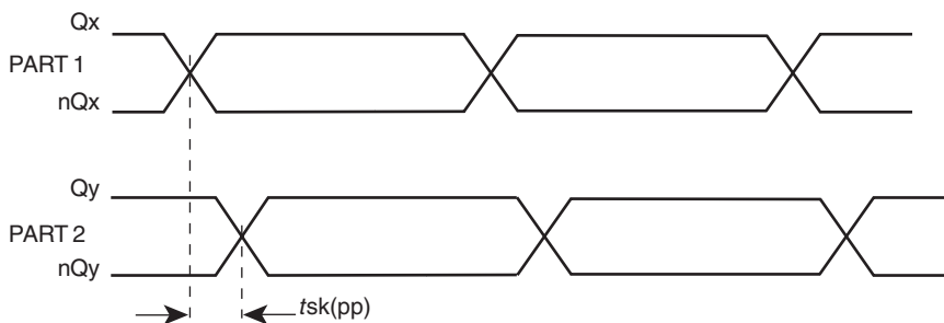
FIGURE 5 - PART-TO-PART SKEW
