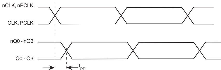
FIGURE 7 - PROPAGATION DELAY
