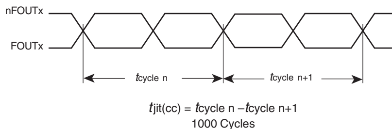
FIGURE 7 - Cycle-to-Cycle Jitter
