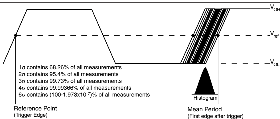
FIGURE 6 - Period Jitter
