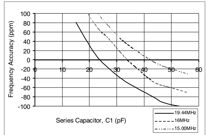
FIGURE 4C. Recommended tuning capacitance for various parallel resonant crystals.
