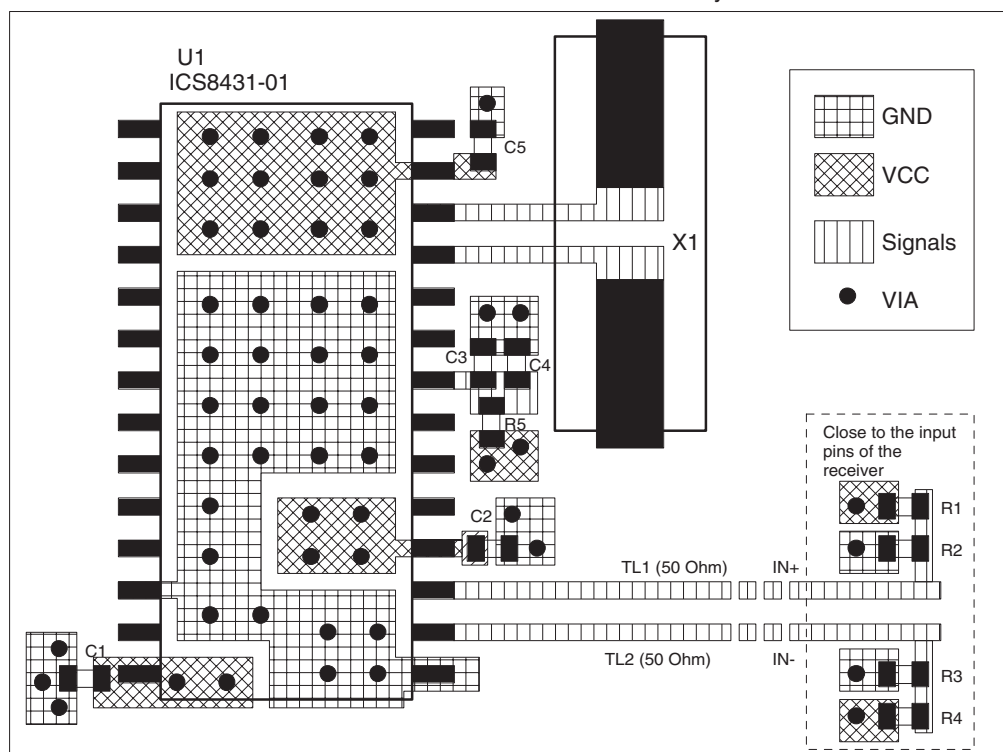
FIGURE 9B - PCB BOARD LAYOUT FOR ICS8431I-01
