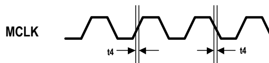
Figure 2. MCLK Timing
