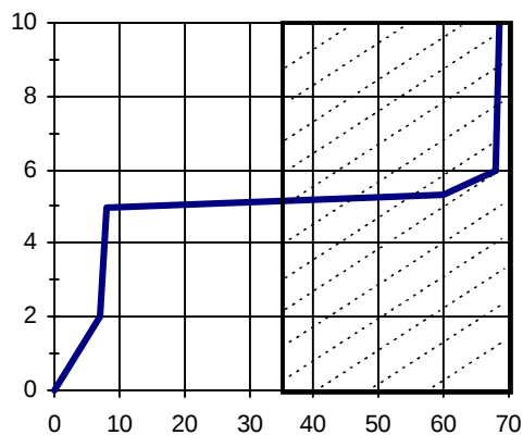
Figure 8 - I_{\text{cc}} (mA) vs V_{\text{cc}}-V_{\text{in}} (V)
