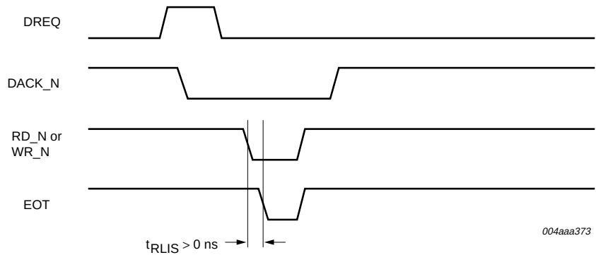
Fig 38. External EOT timing for single-cycle DMA.
