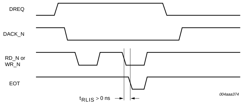
Fig 39. External EOT timing for burst mode DMA.
