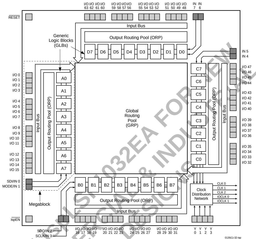
Figure 1. ispLSI 1032 Functional Block Diagram
