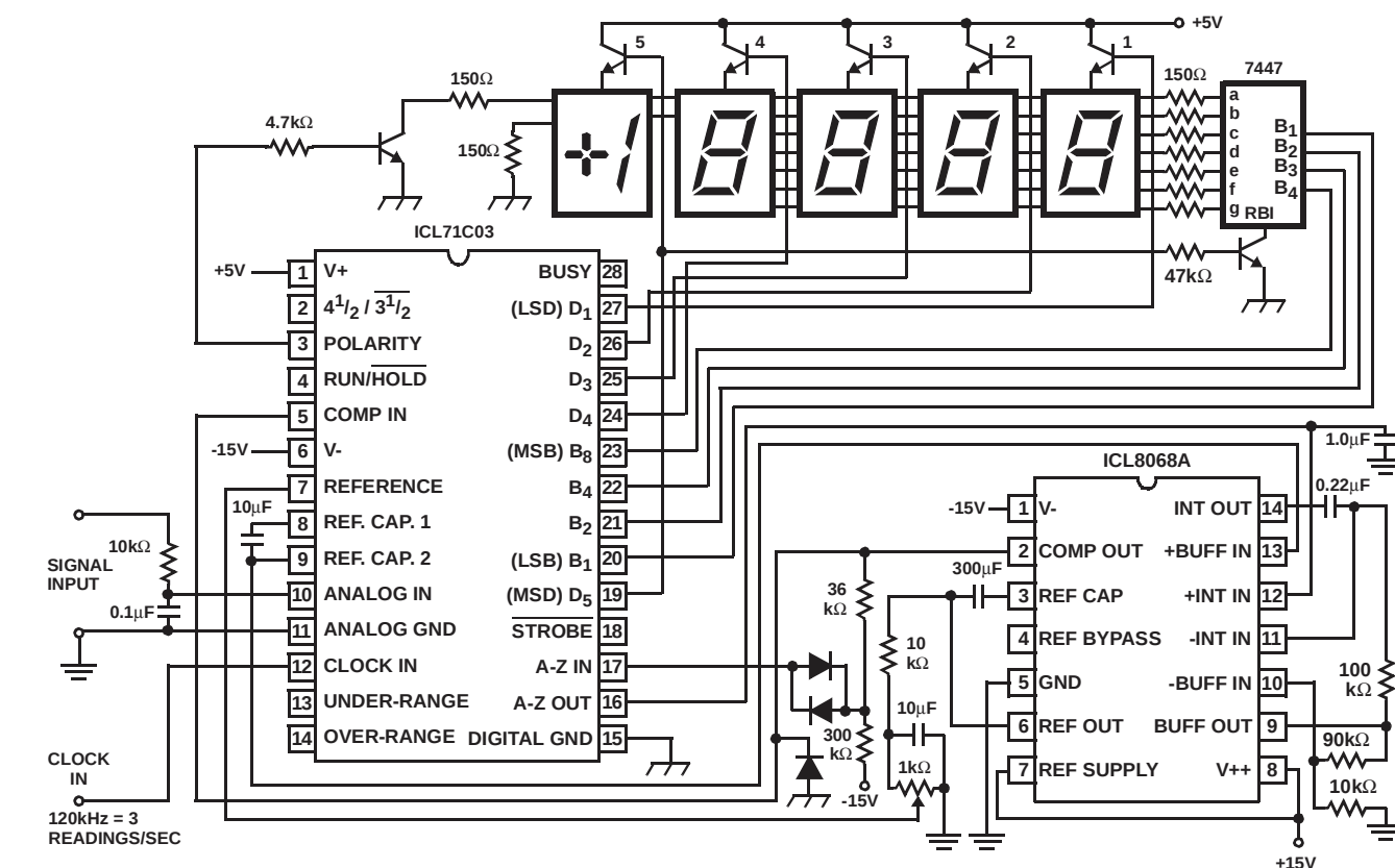
FIGURE 7. ICL8052A (8068A)/71C03A 4\frac{1}{2} DIGIT A/D CONVERTER
