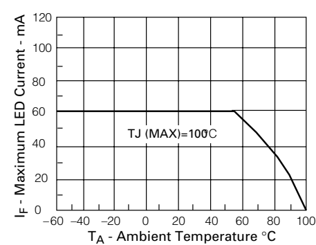
Figure 5. Maximum LED current versus ambient temperature
