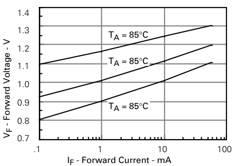
Figure 7. Forward voltage versus forward current
