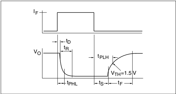
Figure 3. Saturated switching timing
