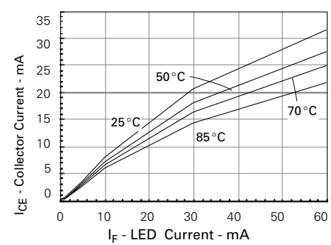
Figure 8. Collector-emitter current versus temperature and LED current
