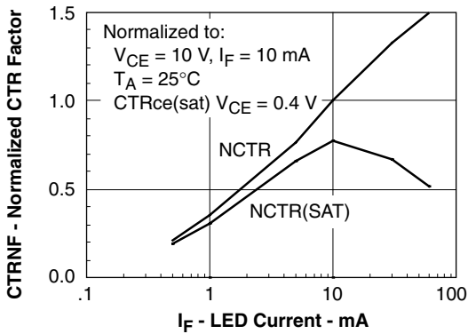
Figure 6. Normalized non-saturated and saturated CTR at T_A=25^\circ C versus LED current
