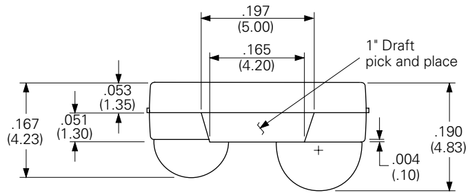
Figure 9. IRMS6100/IRMT6100 Detail Drawings With Optional Side View or Top View Mounting
