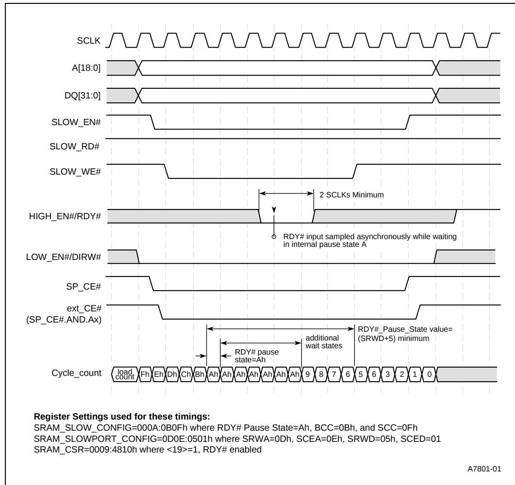
Figure 73. SRAM SlowPort RDY#
