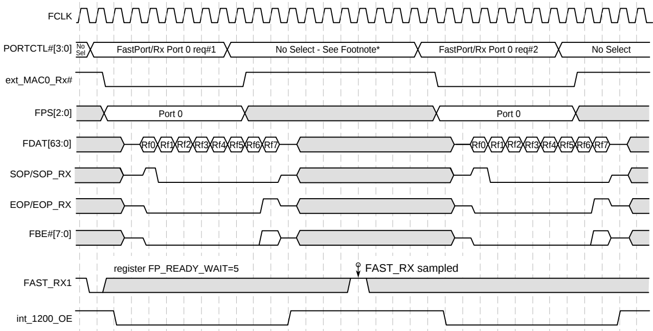
Figure 48. 64-Bit Bidirectional Ix Bus Timing - Consecutive FastPort Receives, Same Port, EOP, No Status, FP_READY_WAIT=5
