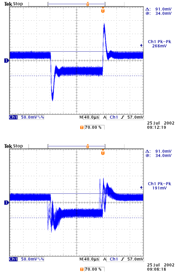
FIGURE 25. SAMPLE OUTPUT VOLTAGE TRANSIENT RESPONSE WITHOUT & WITH ATR ENGAGED
