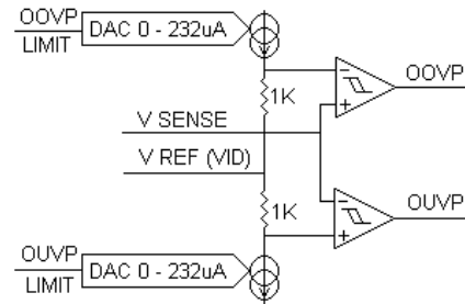
FIGURE 28. OOVP OUVP WINDOW COMPARATOR
