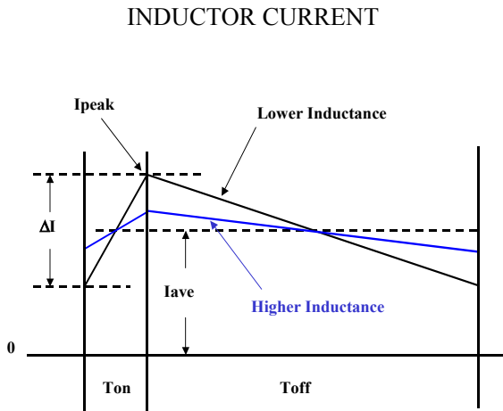
FIGURE 32. AFFECT OF INDUCTANCE ON PEAK CURRENT
