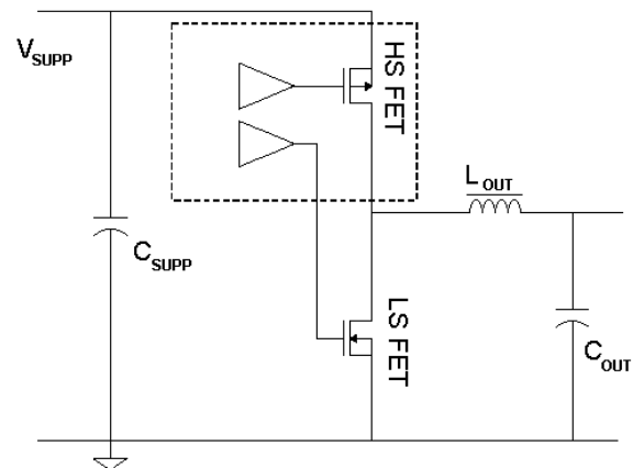
FIGURE 38. SYNCHRONOUS BUCK CONVERTER USING ISL6580
