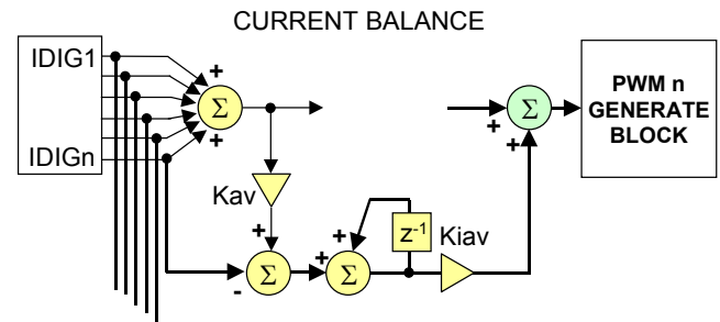
FIGURE 10. CURRENT BALANCE
