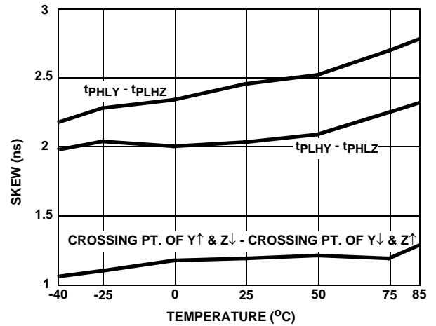
FIGURE 11. DRIVER SKEW vs TEMPERATURE (ISL8485, ISL8490, ISL8491)
