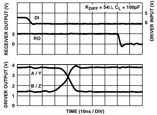
FIGURE 13. DRIVER AND RECEIVER WAVEFORMS, HIGH TO LOW (ISL8485, ISL8490, ISL8491)
