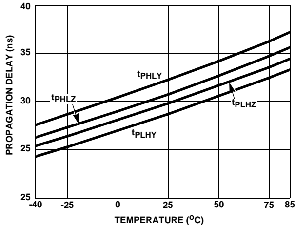
FIGURE 10. DRIVER PROPAGATION DELAY vs TEMPERATURE (ISL8485, ISL8490, ISL8491)
