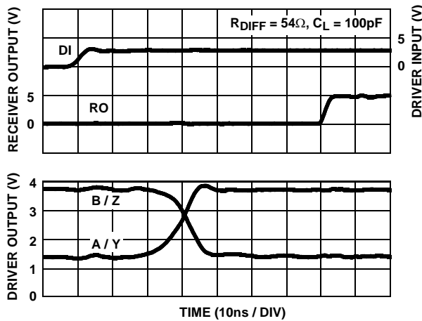
FIGURE 12. DRIVER AND RECEIVER WAVEFORMS, LOW TO HIGH (ISL8485, ISL8490, ISL8491)
