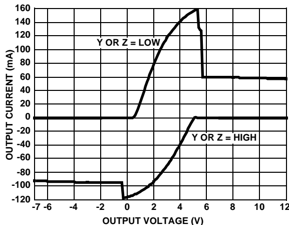
FIGURE 8. DRIVER OUTPUT CURRENT vs SHORT CIRCUIT VOLTAGE
