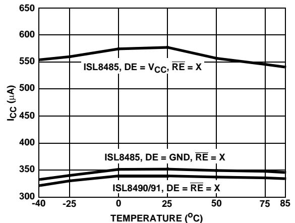
FIGURE 9. SUPPLY CURRENT vs TEMPERATURE (ISL8485, ISL8490, ISL8491)
