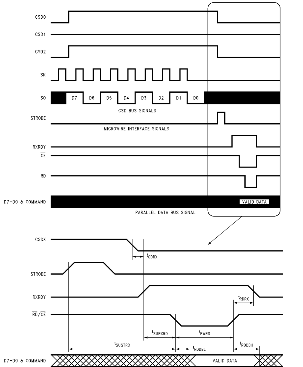
FIGURE 15. Host Port Read from Digital Chip (ICSS1002)
