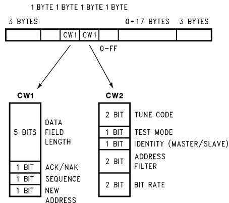
FIGURE 5. Packet Structure
