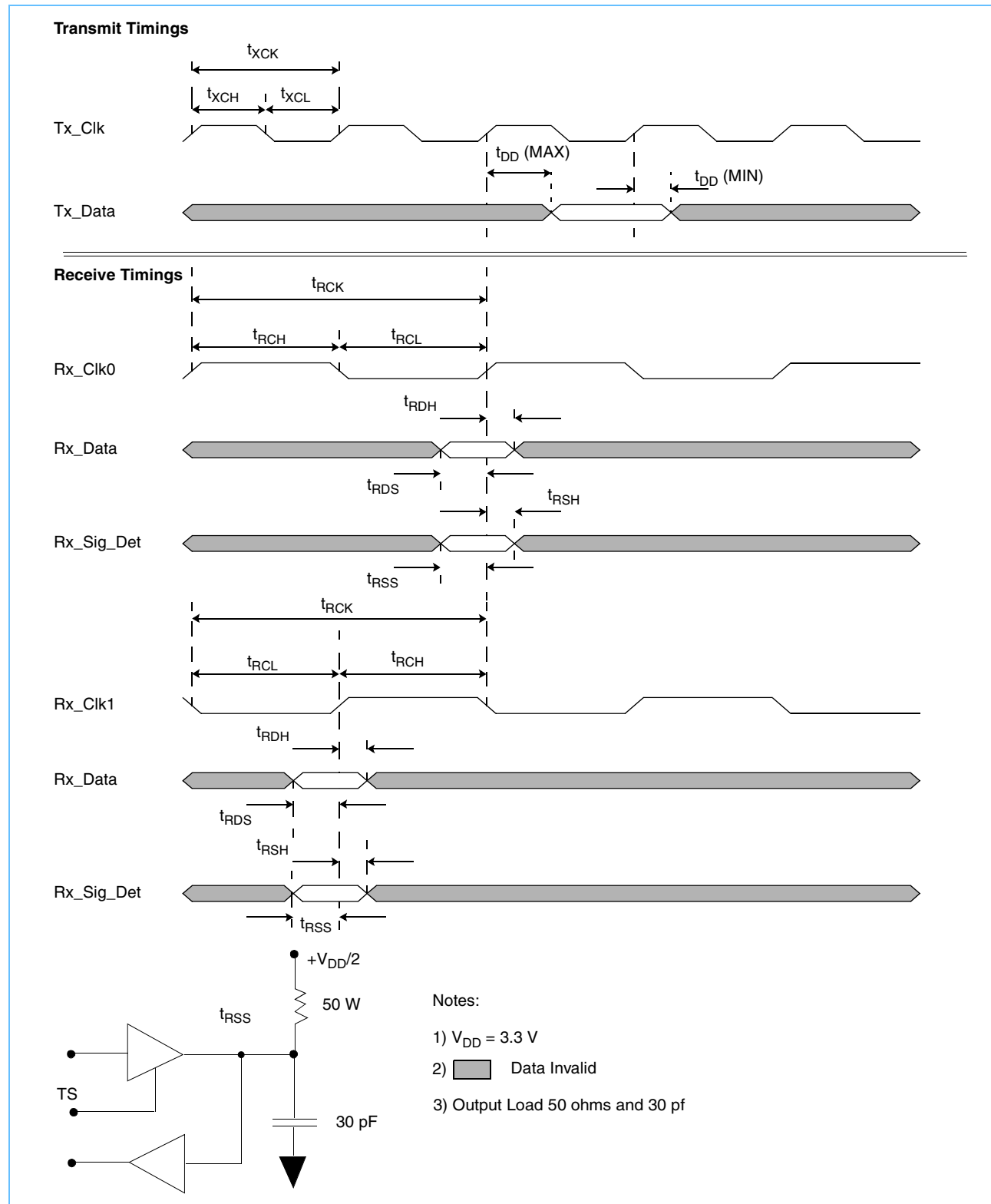
Figure 2-8. TBI Timing Diagram
