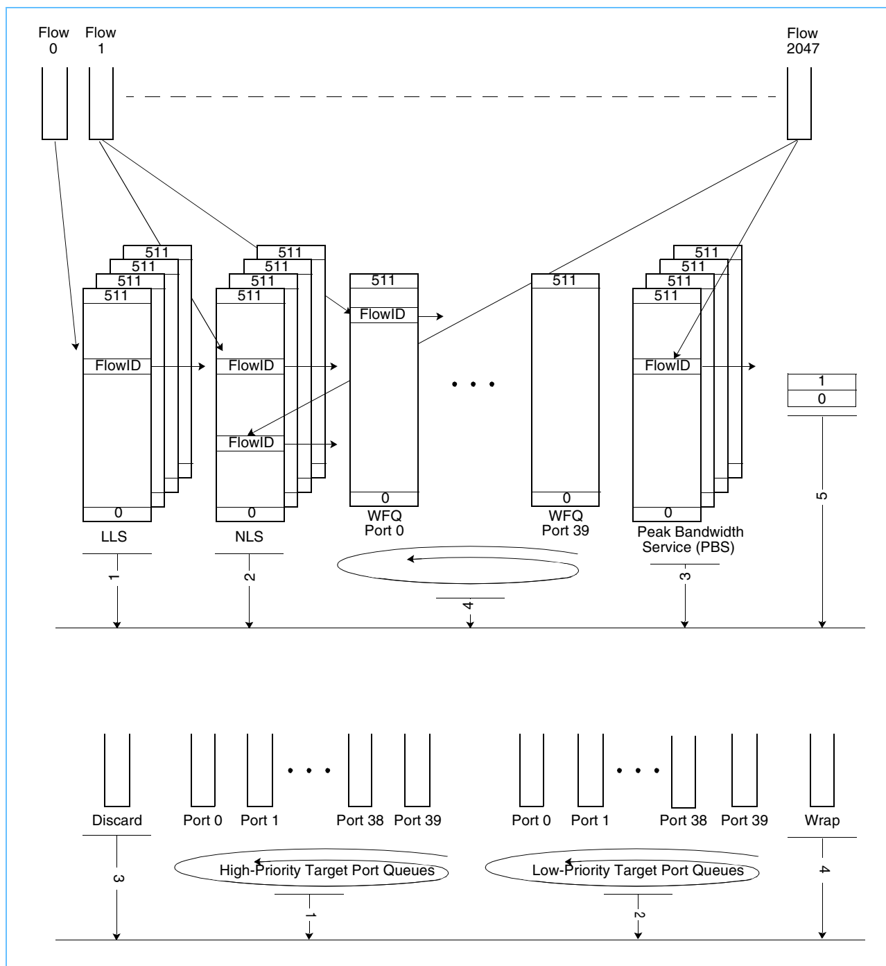
Figure 6-6. The Egress Scheduler
