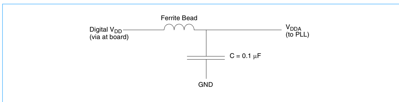
Figure 2-15. PLL Filter Circuit Diagram
