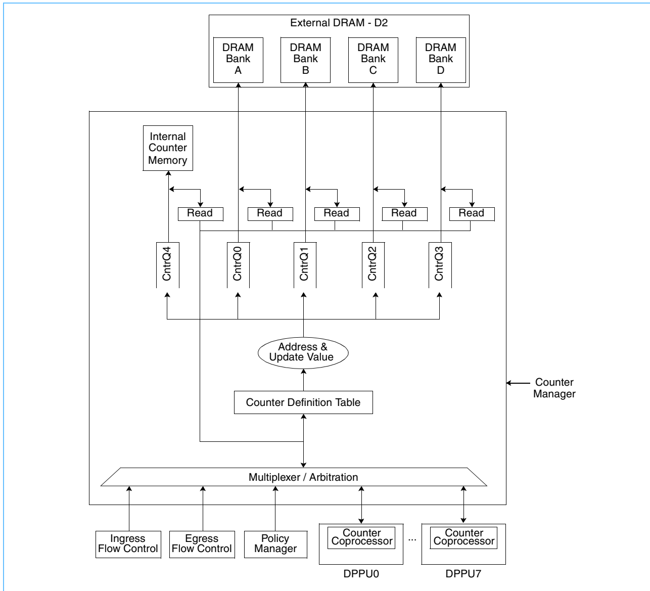
Figure 7-20. Counter Manager Block Diagram
