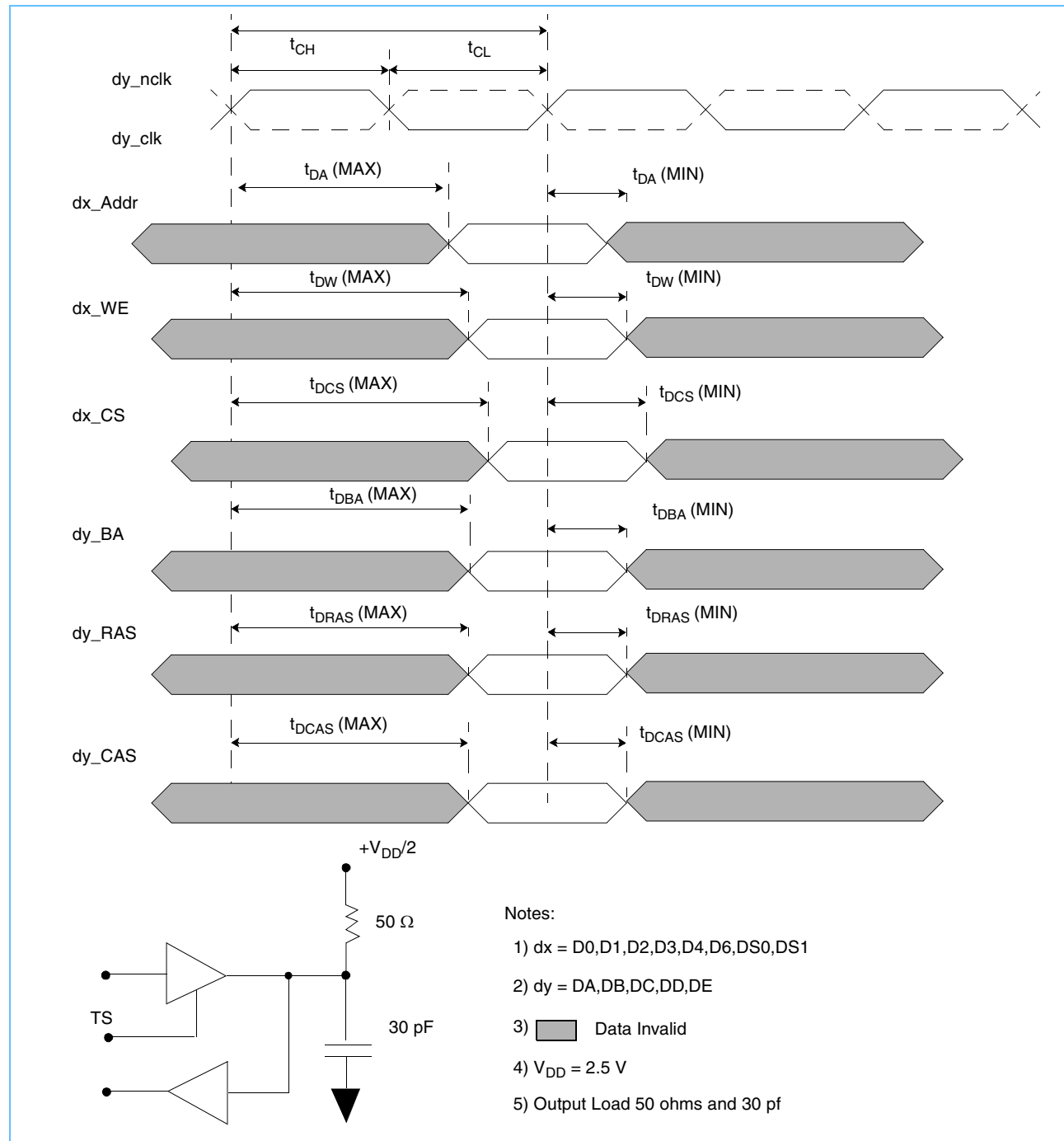
Figure 2-3. DDR Control Timing Diagram
