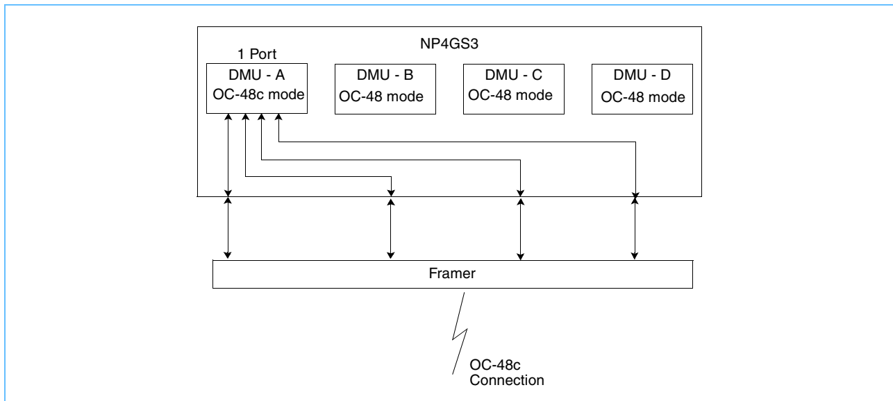
Figure 3-9. OC-48c Configuration
