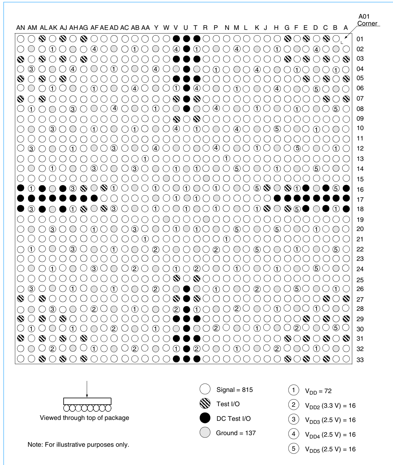
Figure 2-18. Pins Diagram
