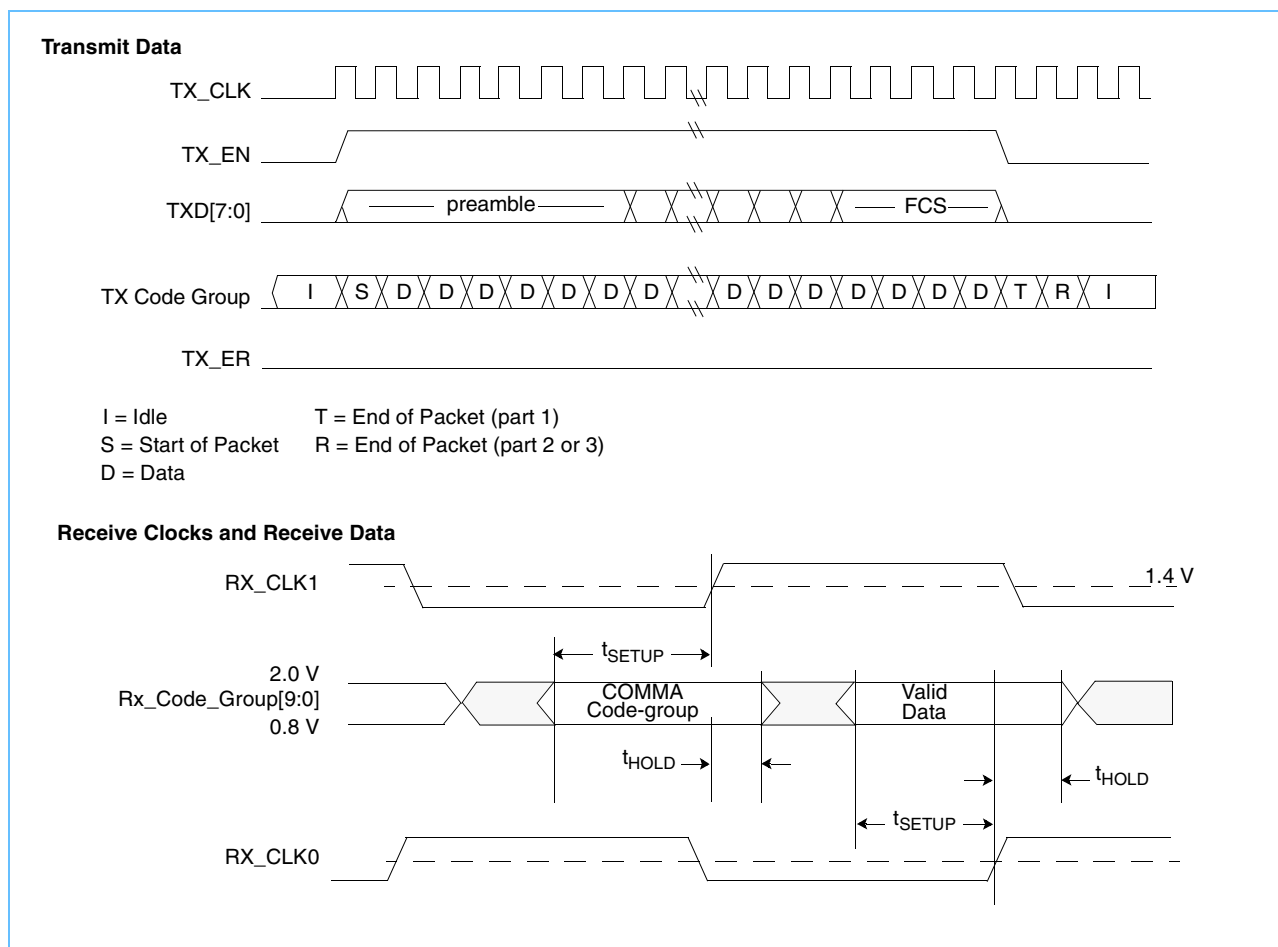
Figure 3-5. TBI Timing Diagram
