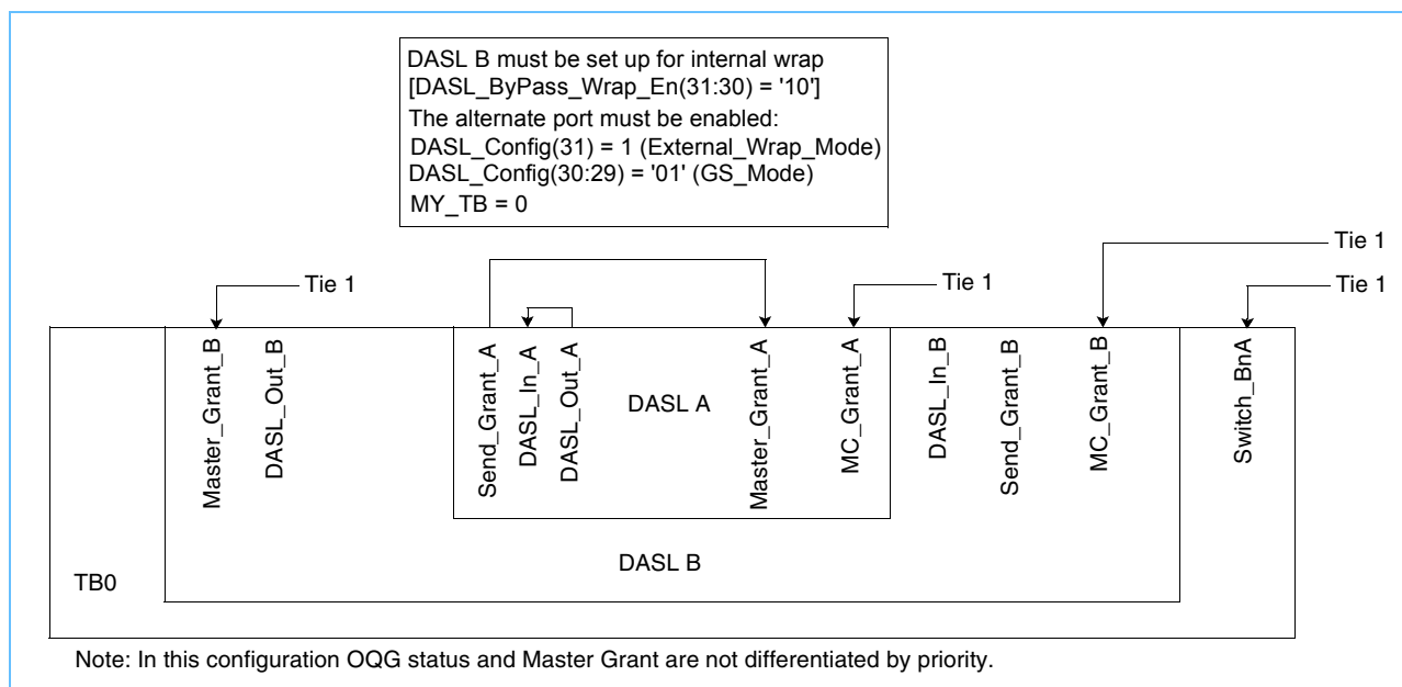
Figure 5-6. External Wrap Mode (single NP4GS3 configuration)
