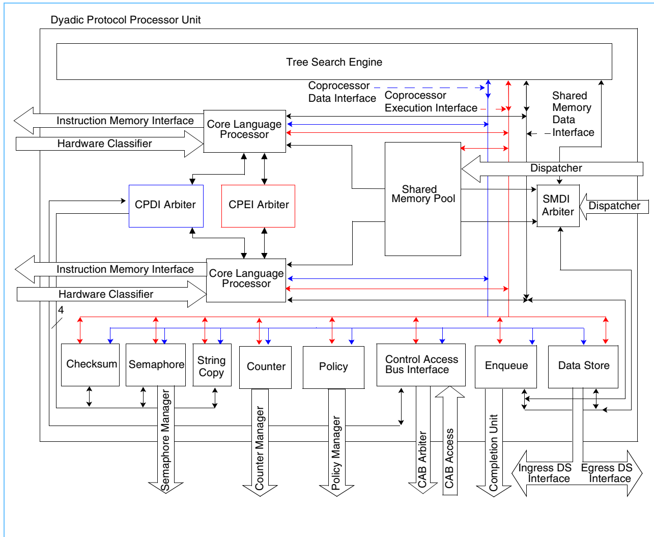
Figure 7-3. Dyadic Protocol Processor Unit Functional Blocks (NP4GS3B (R2.0))
