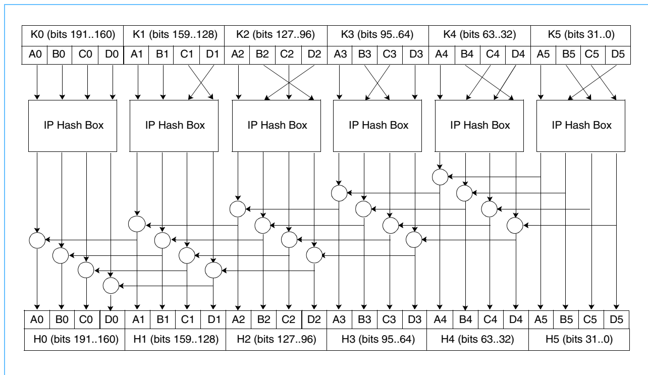
Figure 8-10. 192-Bit IP Hash Function
