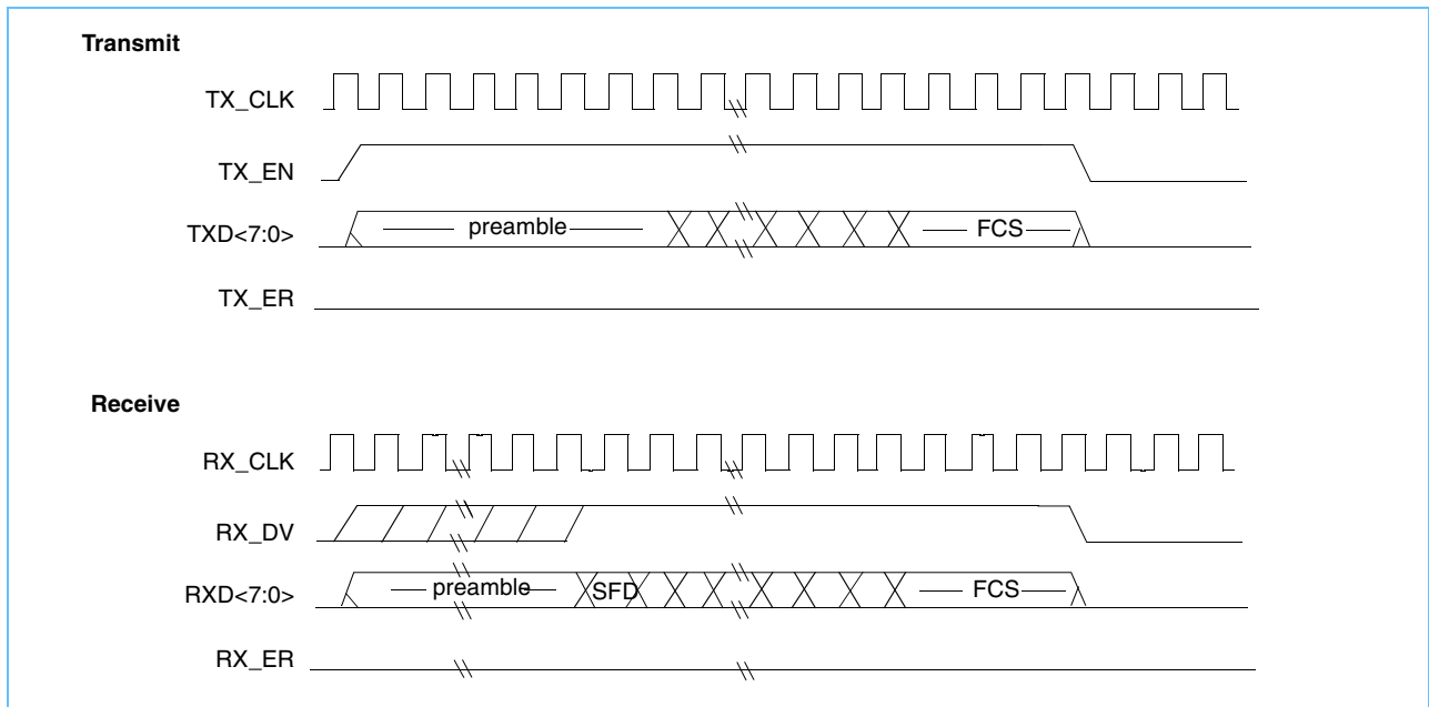
Figure 3-4. GMII Timing Diagram
