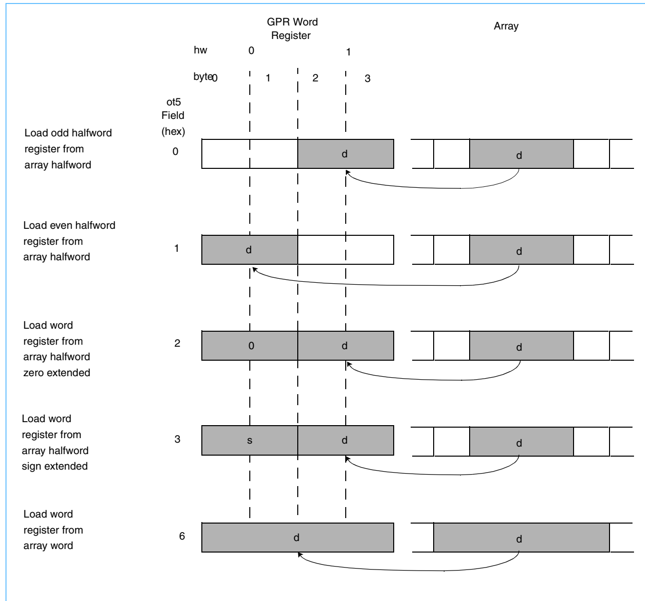
Figure 7-5. ot5 Field Definition: Loading Halfword/Word GPRs from a Halfword/Word Array
