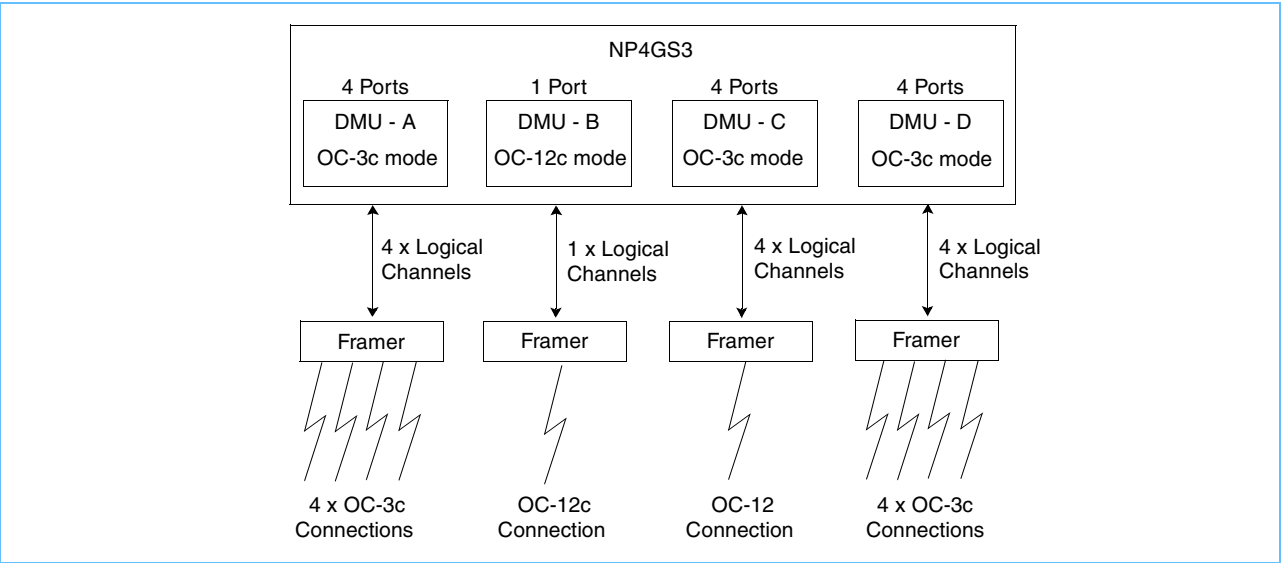
Figure 3-7. OC-3c / OC-12 / OC-12c Configuration
