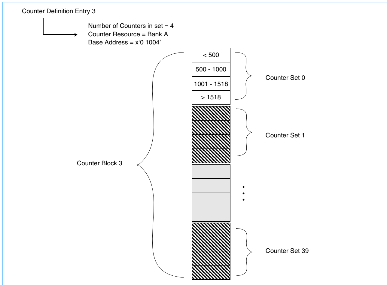
Figure 7-22. Counter Blocks and Sets
