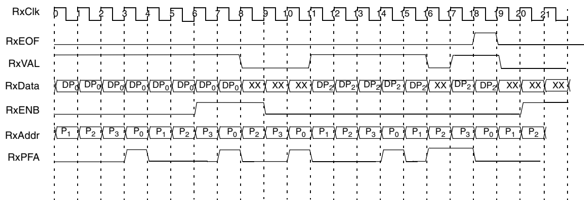
Figure 3-10. Receive POS8 Interface Timing for 8-bit Data Bus (OC-3c)
