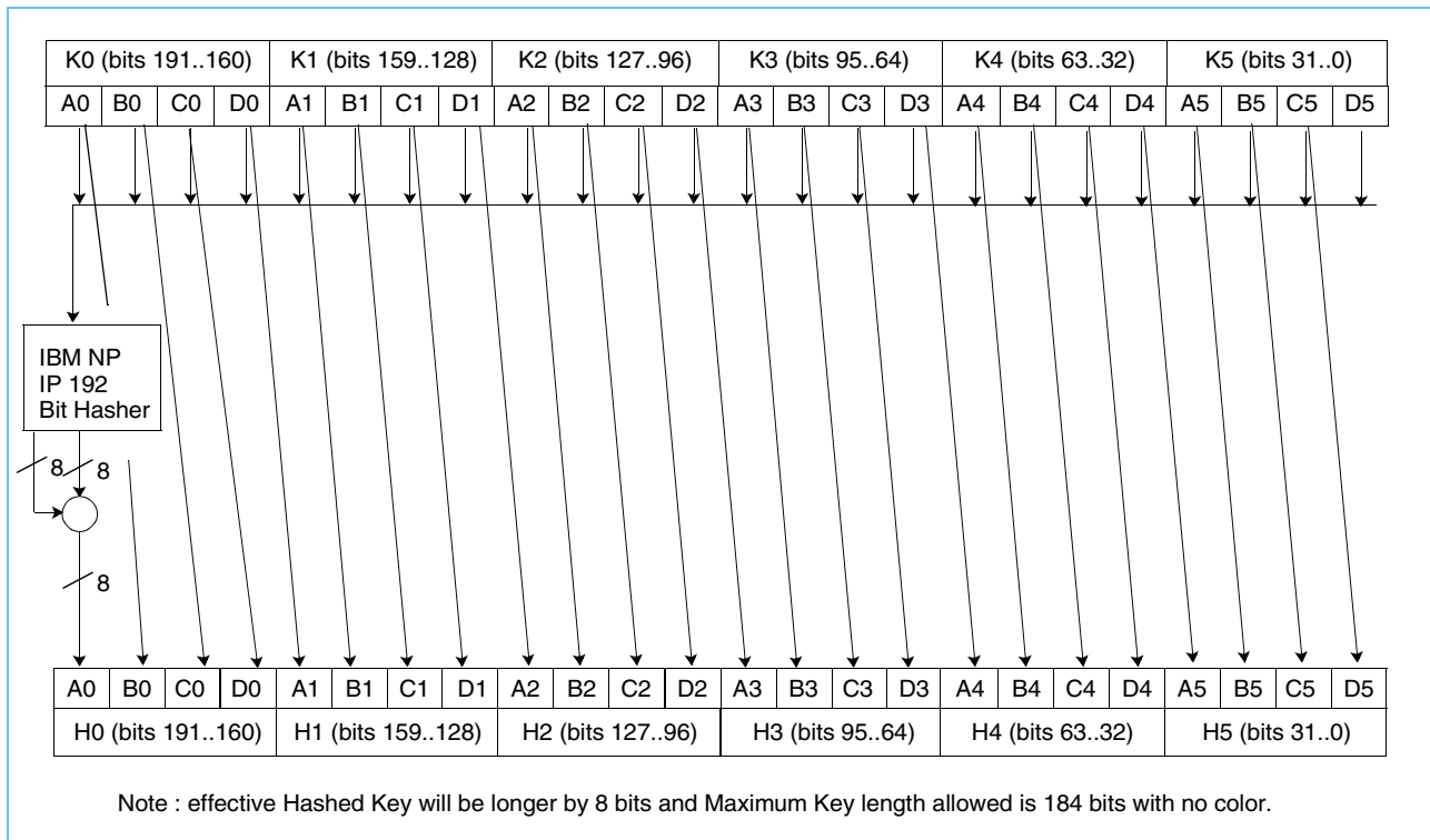
Figure 8-15. 8-bit Hash Function
