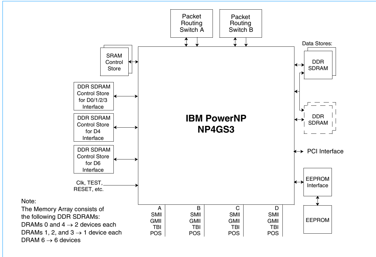
Figure 2-1. Device Interfaces
