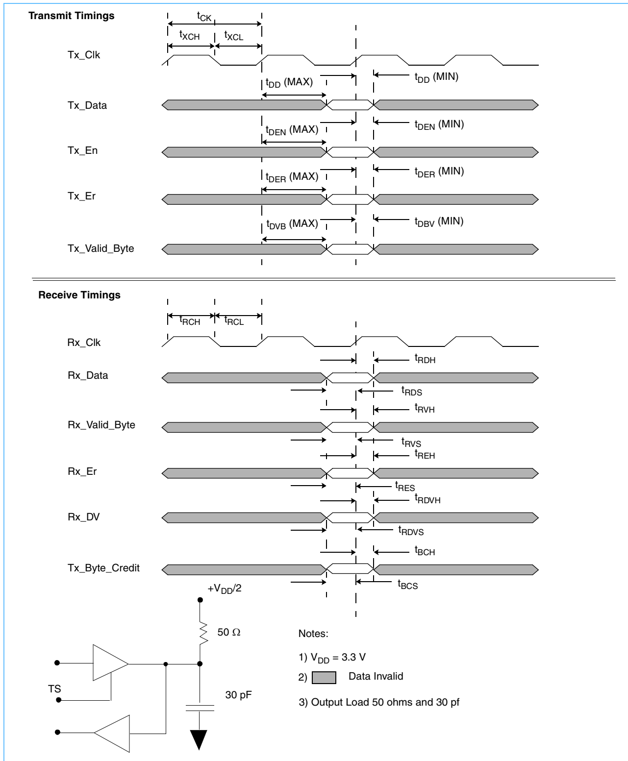
Figure 2-9. GMII Timing Diagram
