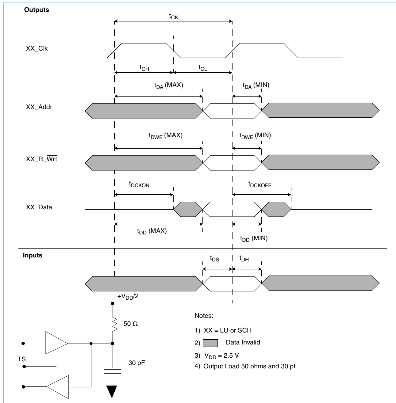
Figure 2-2. ZBT SRAM Timing Diagram
