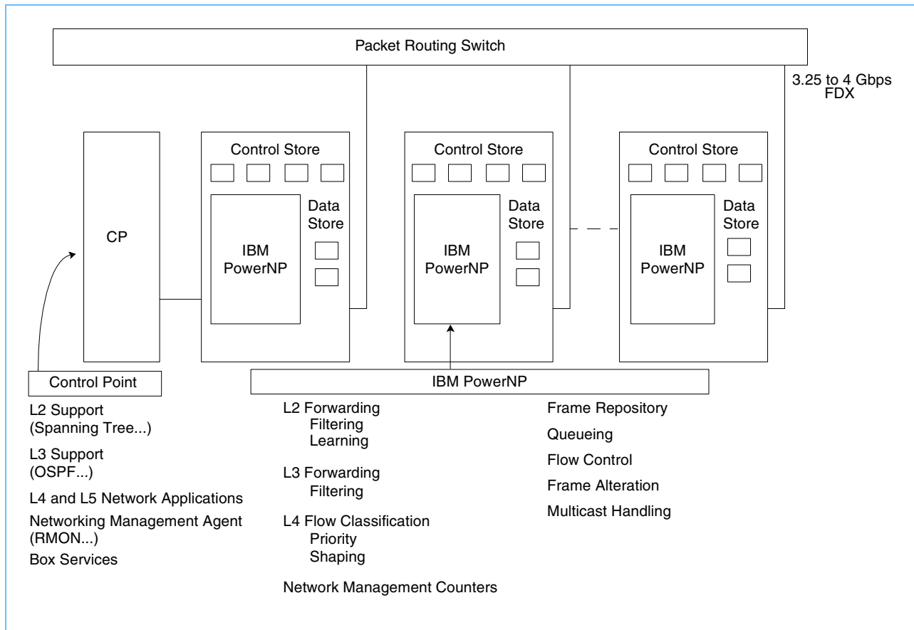
Figure 1-1. Function Placement in an NP4GS3-Based System
