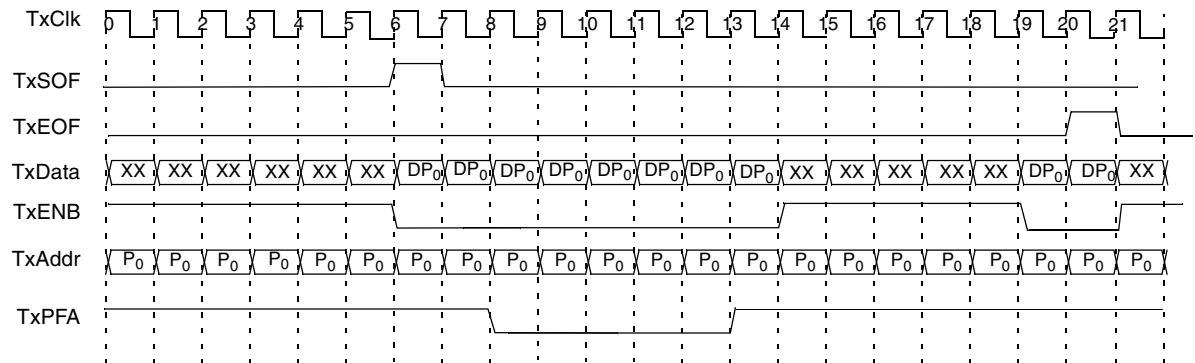
Figure 3-13. Transmit POS8 Interface Timing for 8-bit Data Bus (OC-12c)
