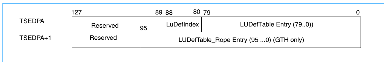
Figure 8-6. General Layout of TSE RDLUDEF in Shared Memory Pool
