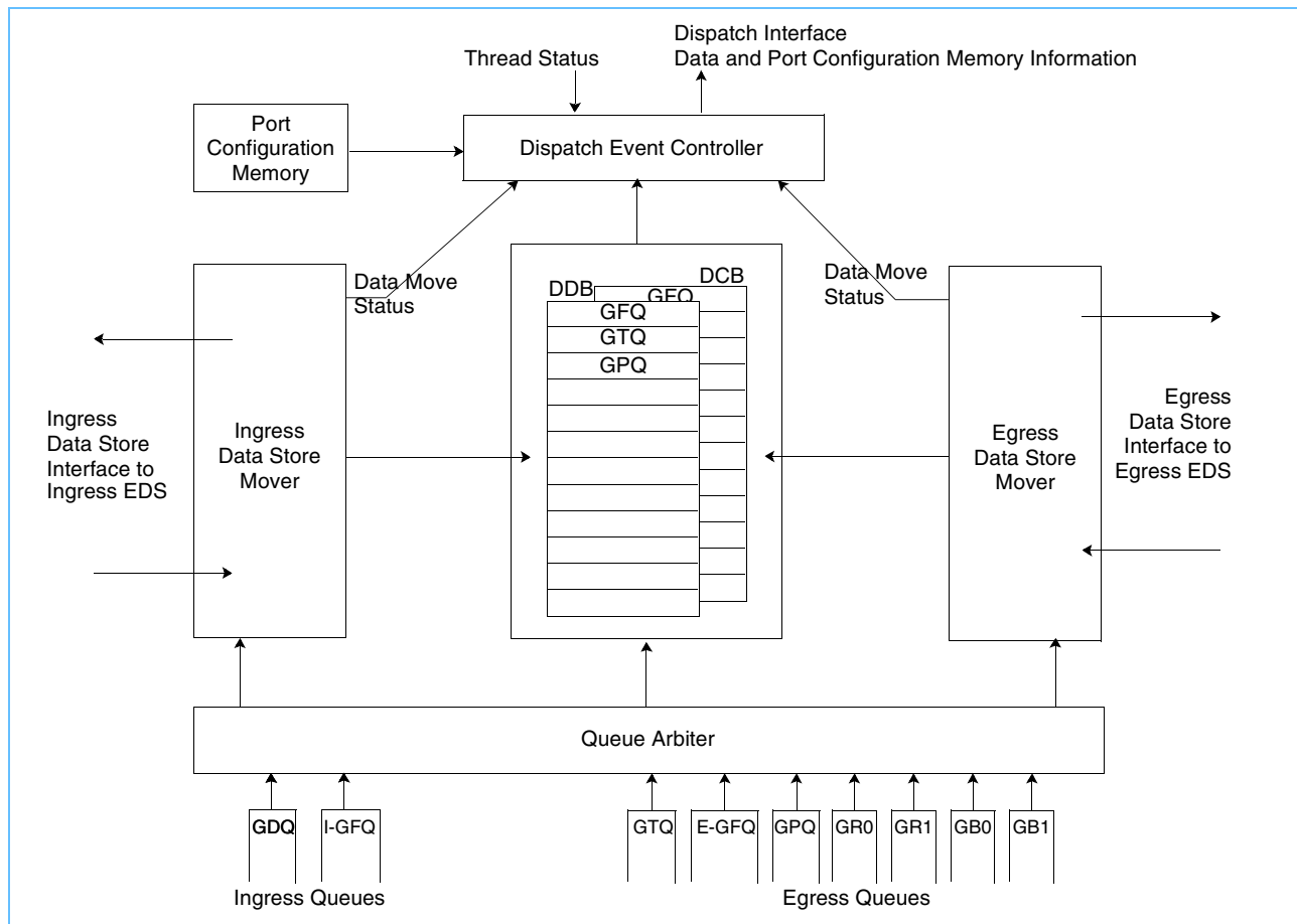
Figure 7-18. Dispatch Unit
