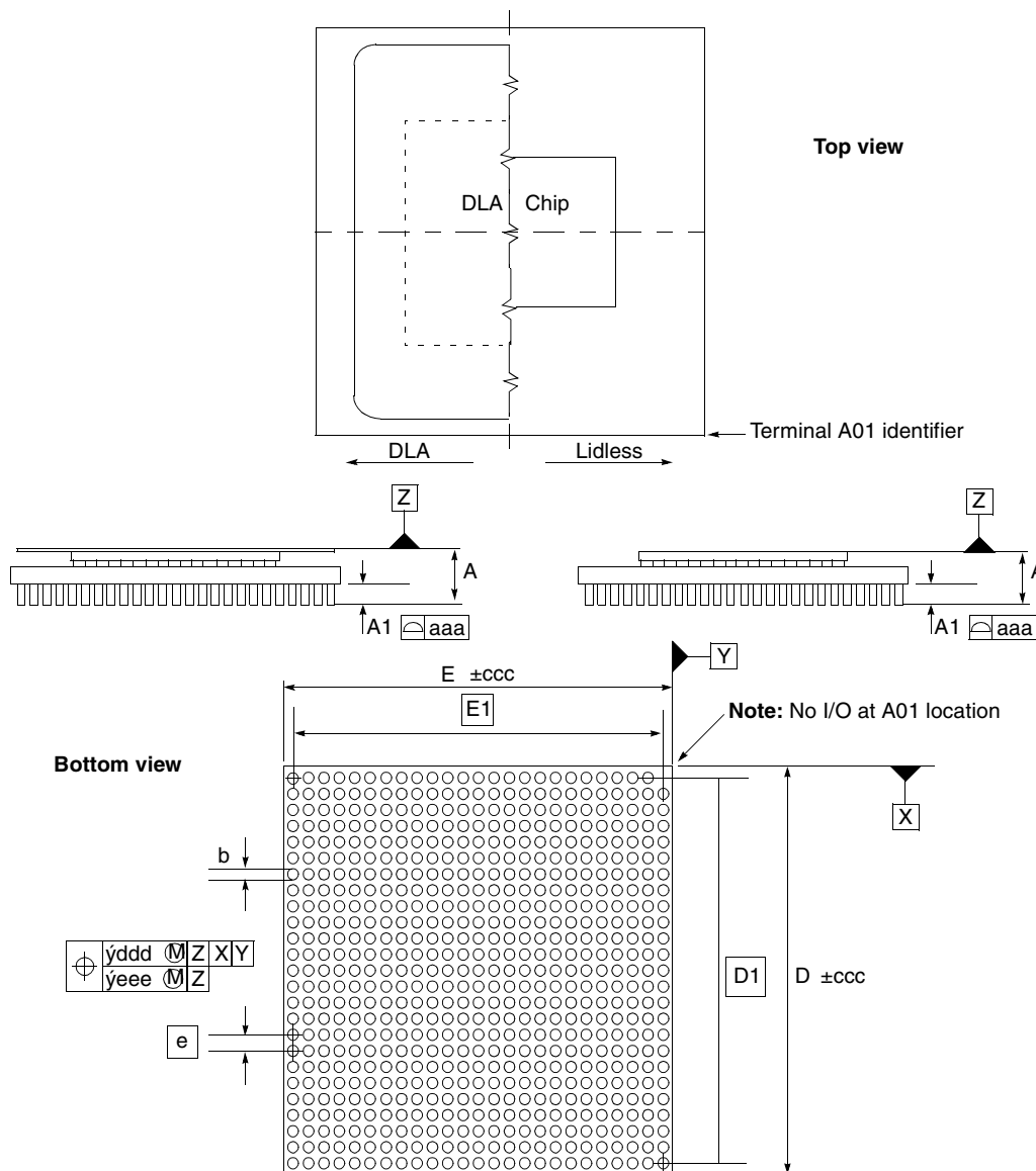
Figure 2-19. Mechanical Diagram
