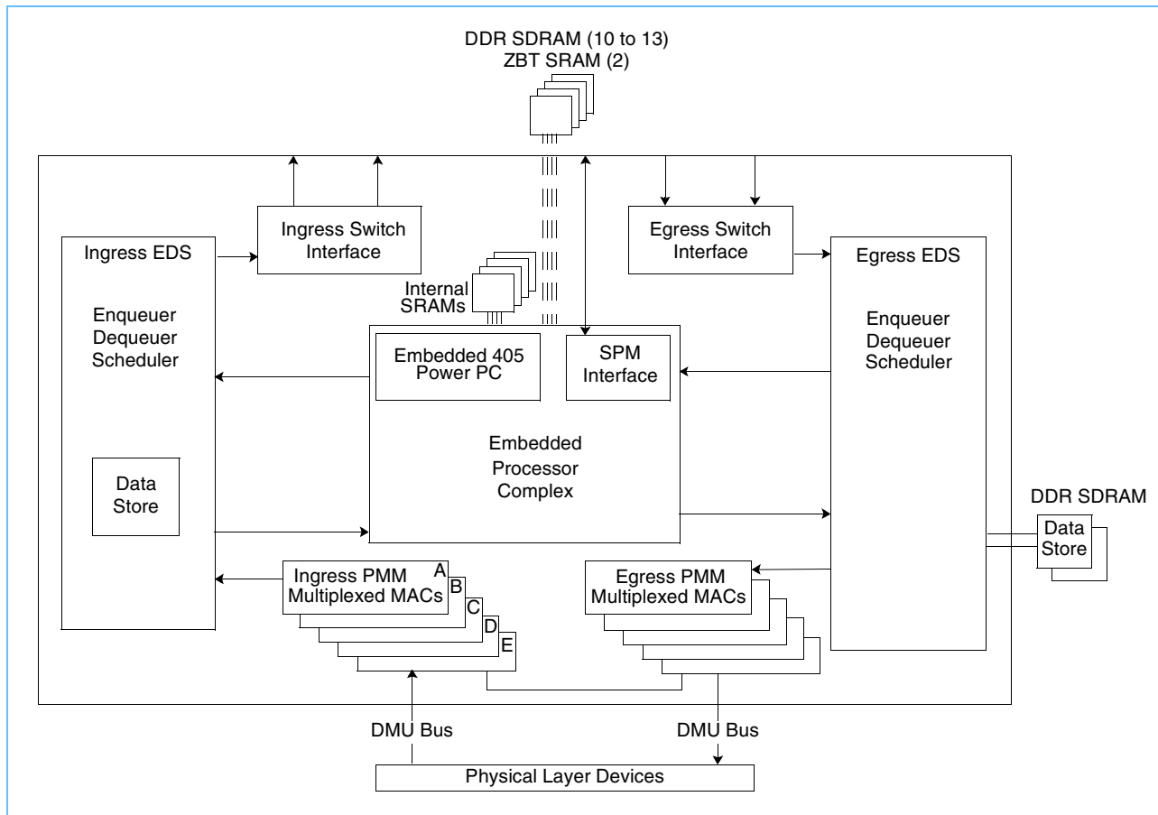
Figure 1-2. NP4GS3 Major Functional Blocks
