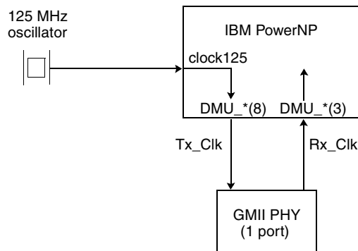
Figure 2-6. NP4GS3 DMU Bus Clock Connections
