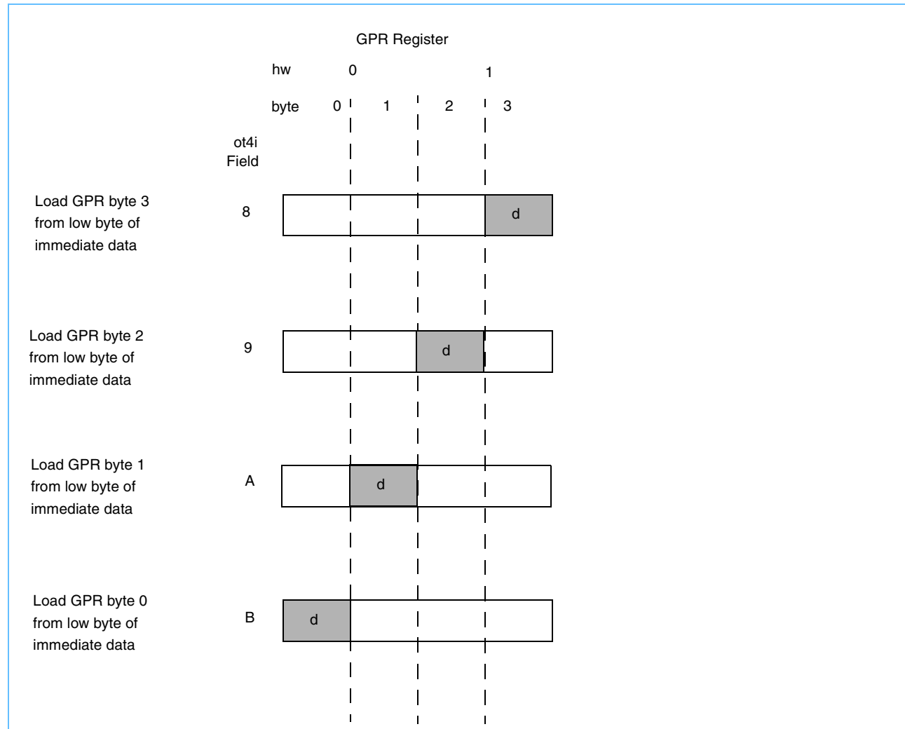
Figure 7-12. ot4i Field Definition: Load Immediate Byte
