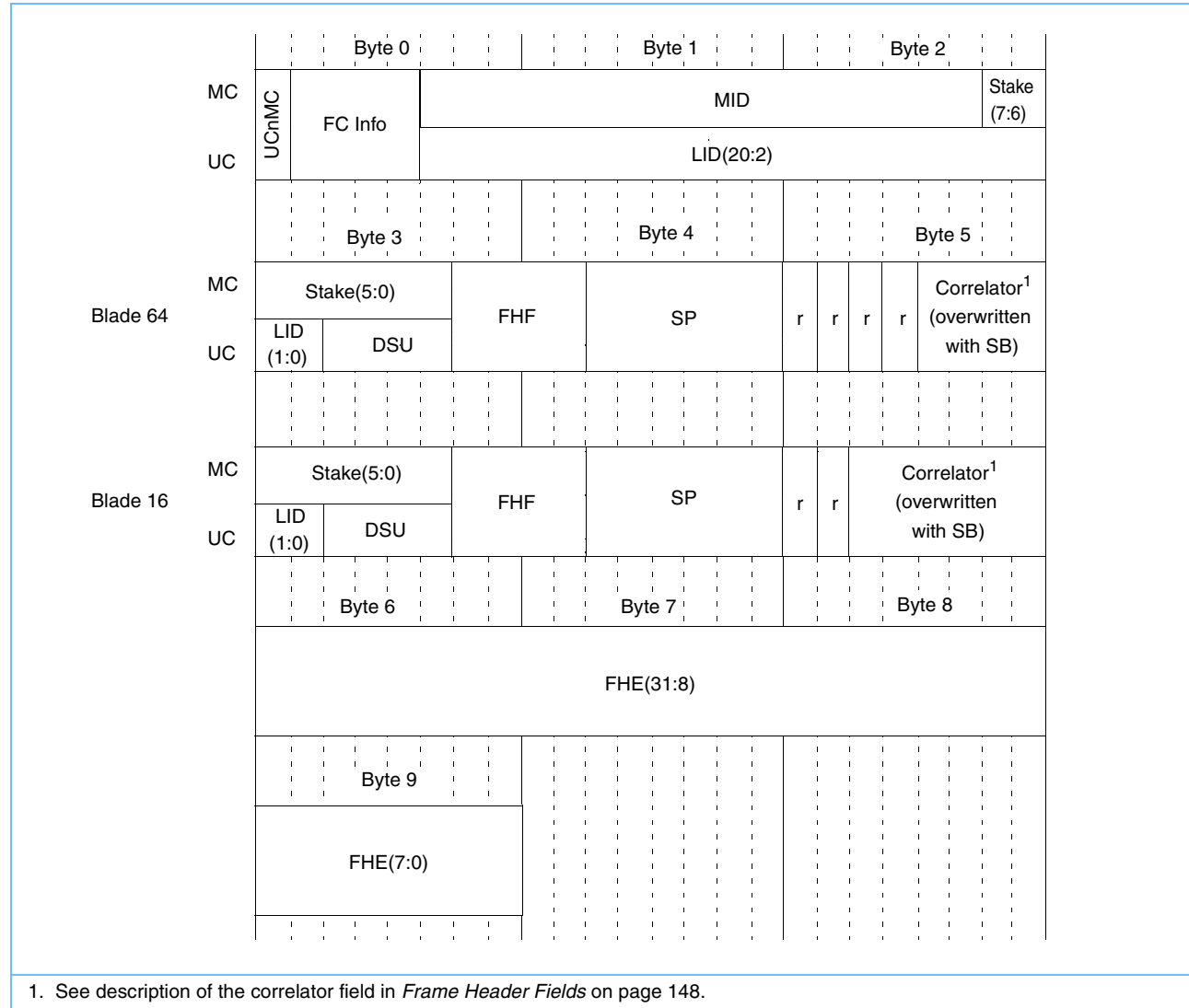
Figure 5-3. Frame Header Format
