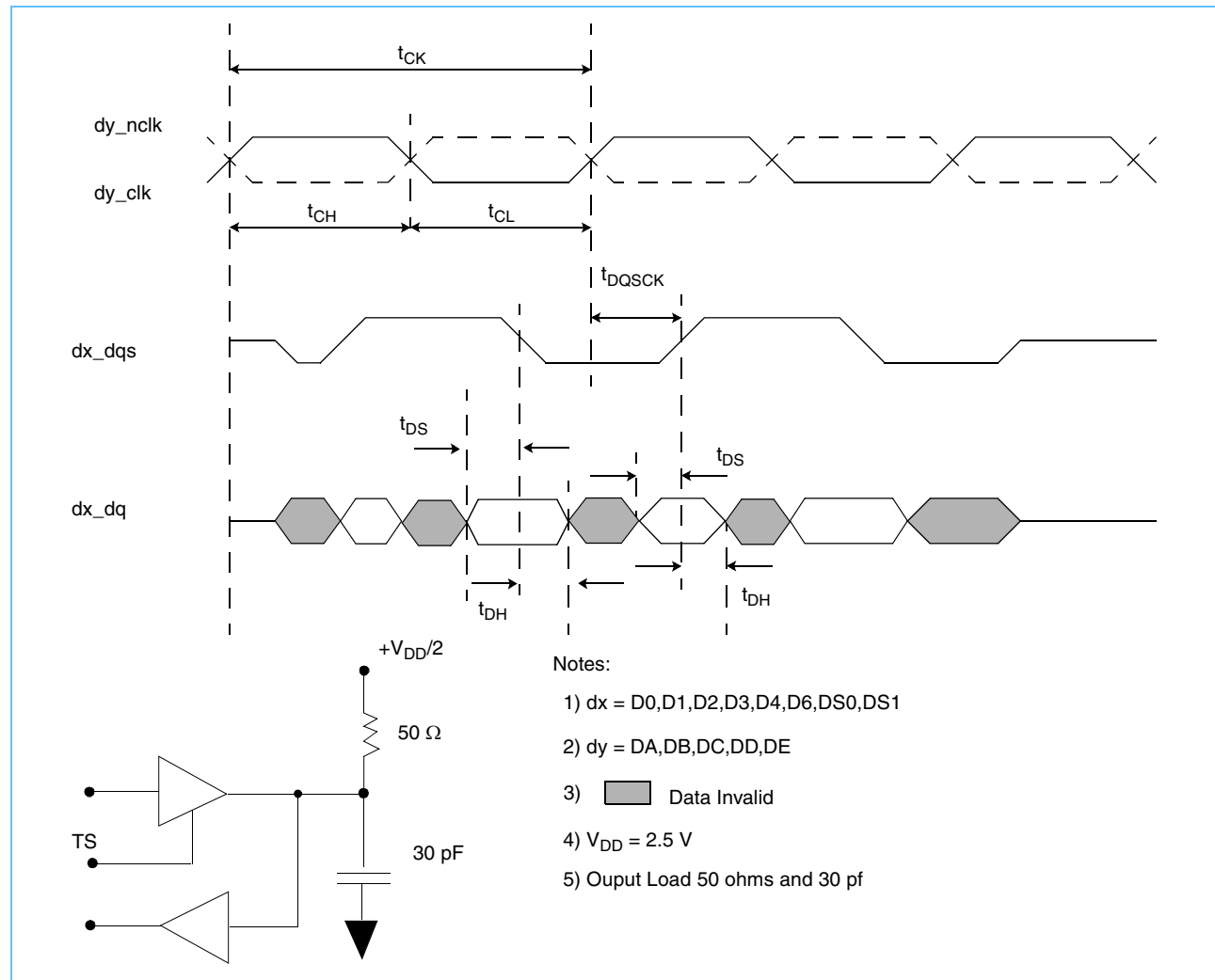
Figure 2-5. DDR Write Output Timing Diagram
