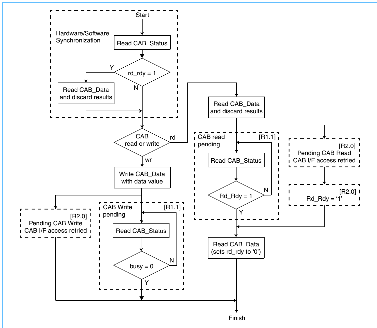
Figure 10-2. Polled Access Flow Diagram
