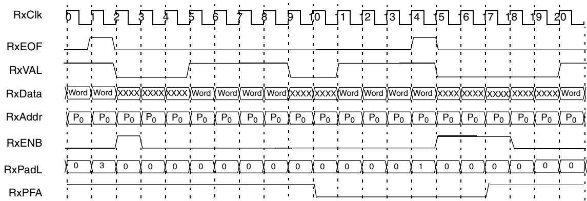
Figure 3-14. Receive POS32 Interface Timing for 32-bit Data Bus (OC-48c)
