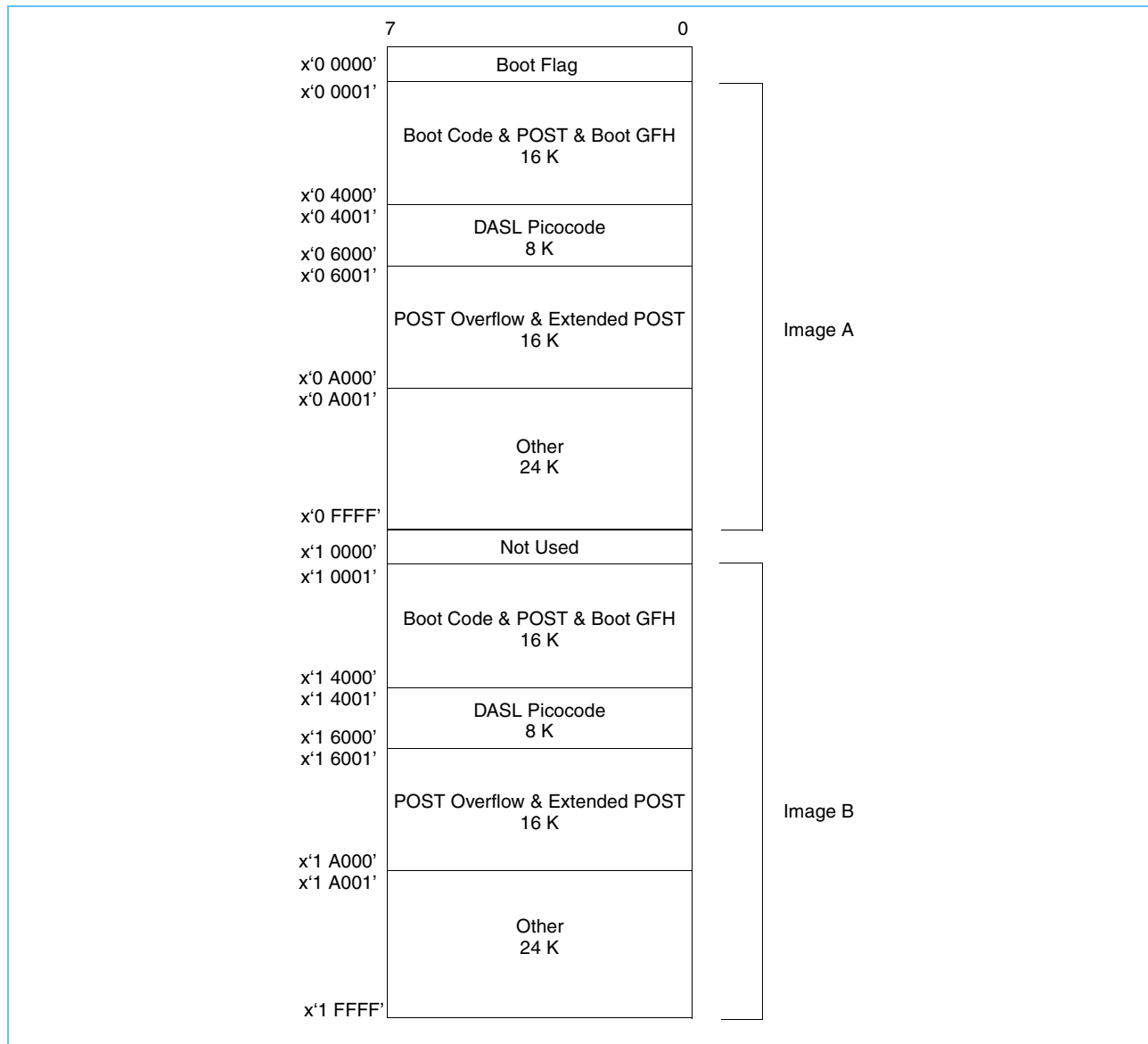
Figure 9-2. EPC Boot Image in External EEPROM
