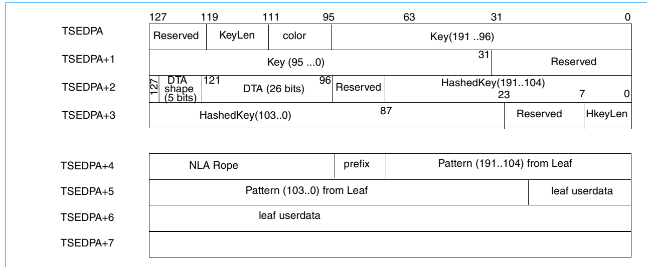
Figure 8-5. General Layout of TSE Fields in Shared Memory Pool
