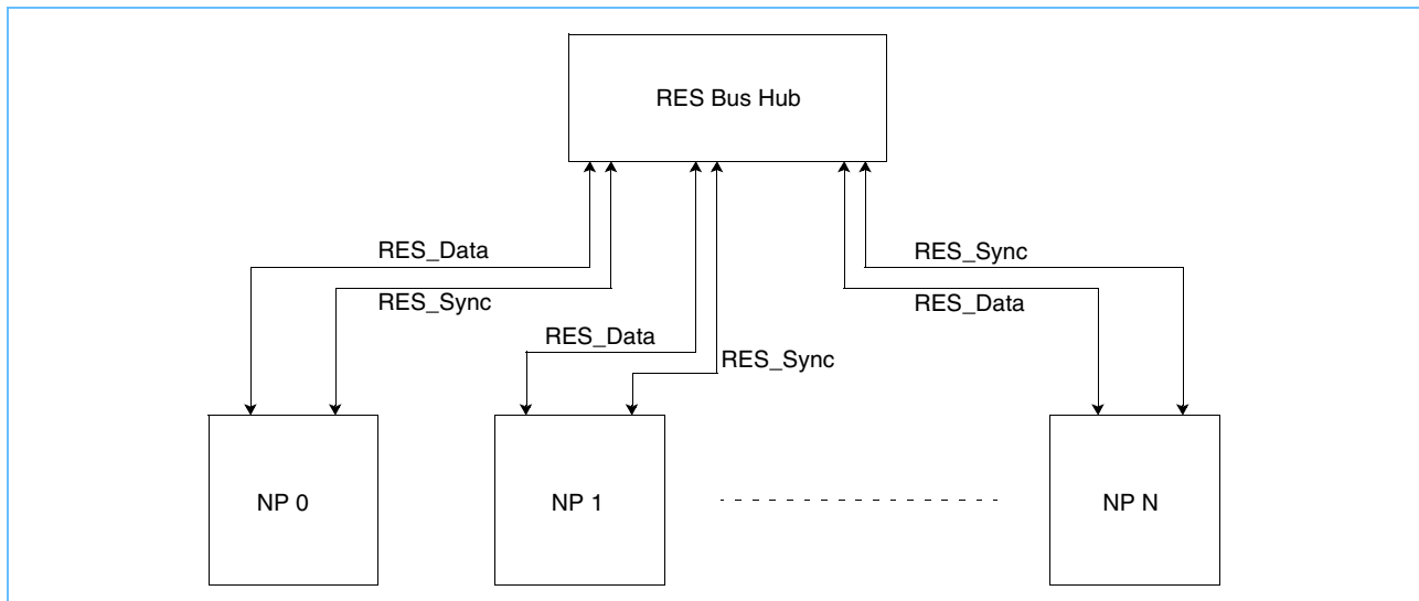
Figure 6-5. Hub-based RES Bus configuration to support more than two NP4GS3s
