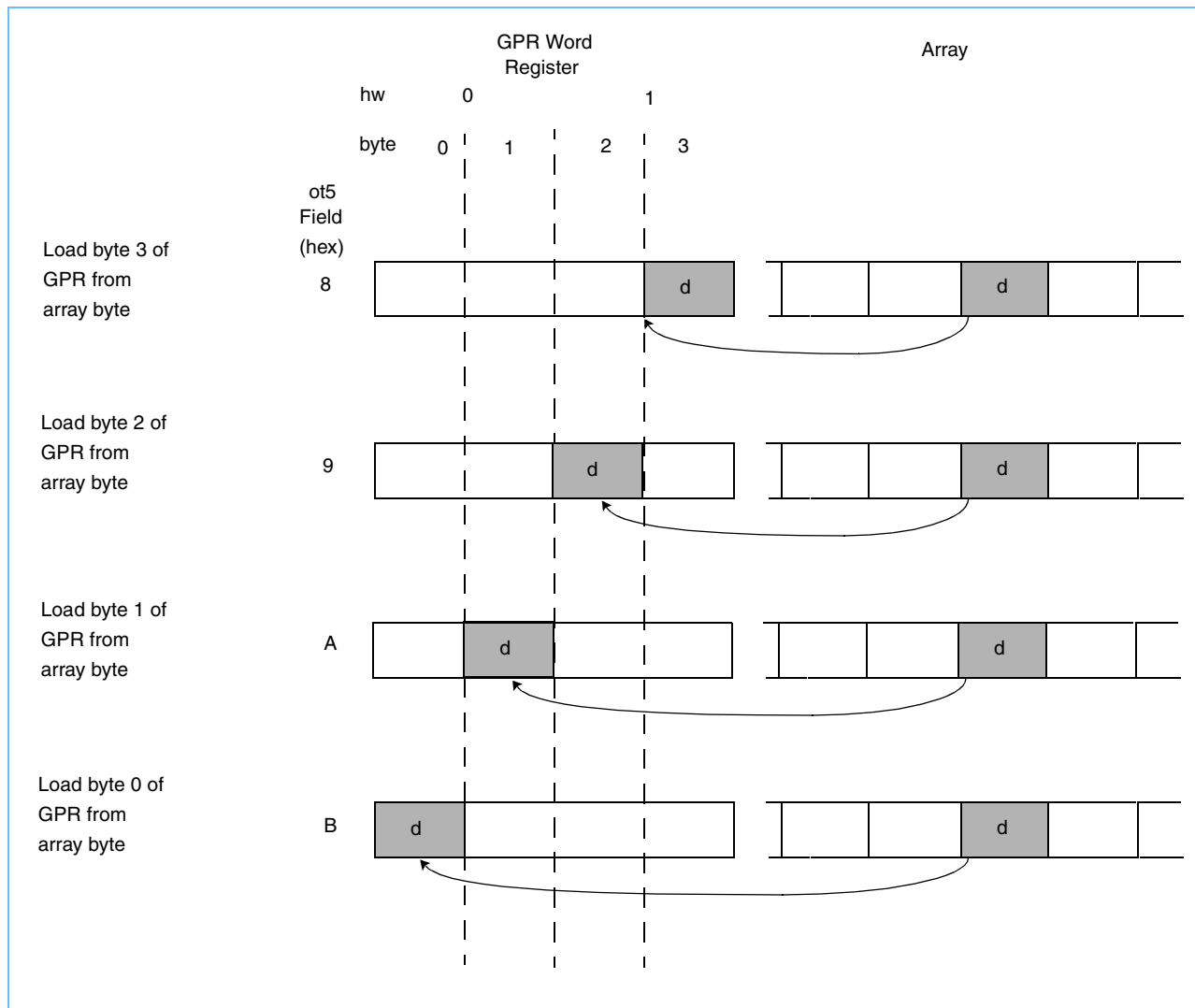
Figure 7-6. ot5 Field Definition: Loading GPR Byte From Array Byte
