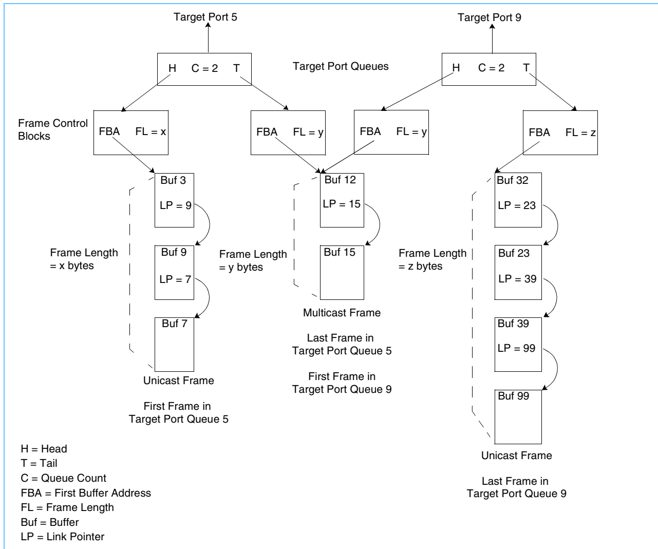
Figure 6-3. TPQ, FCB, and Egress Frame Example
