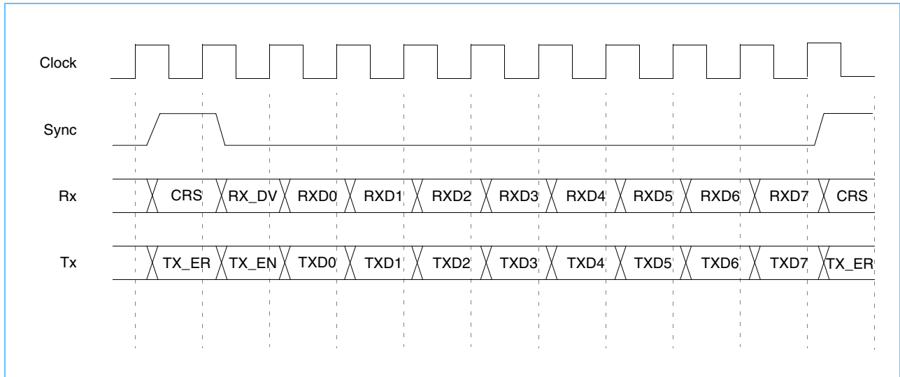
Figure 3-3. SMII Timing Diagram
