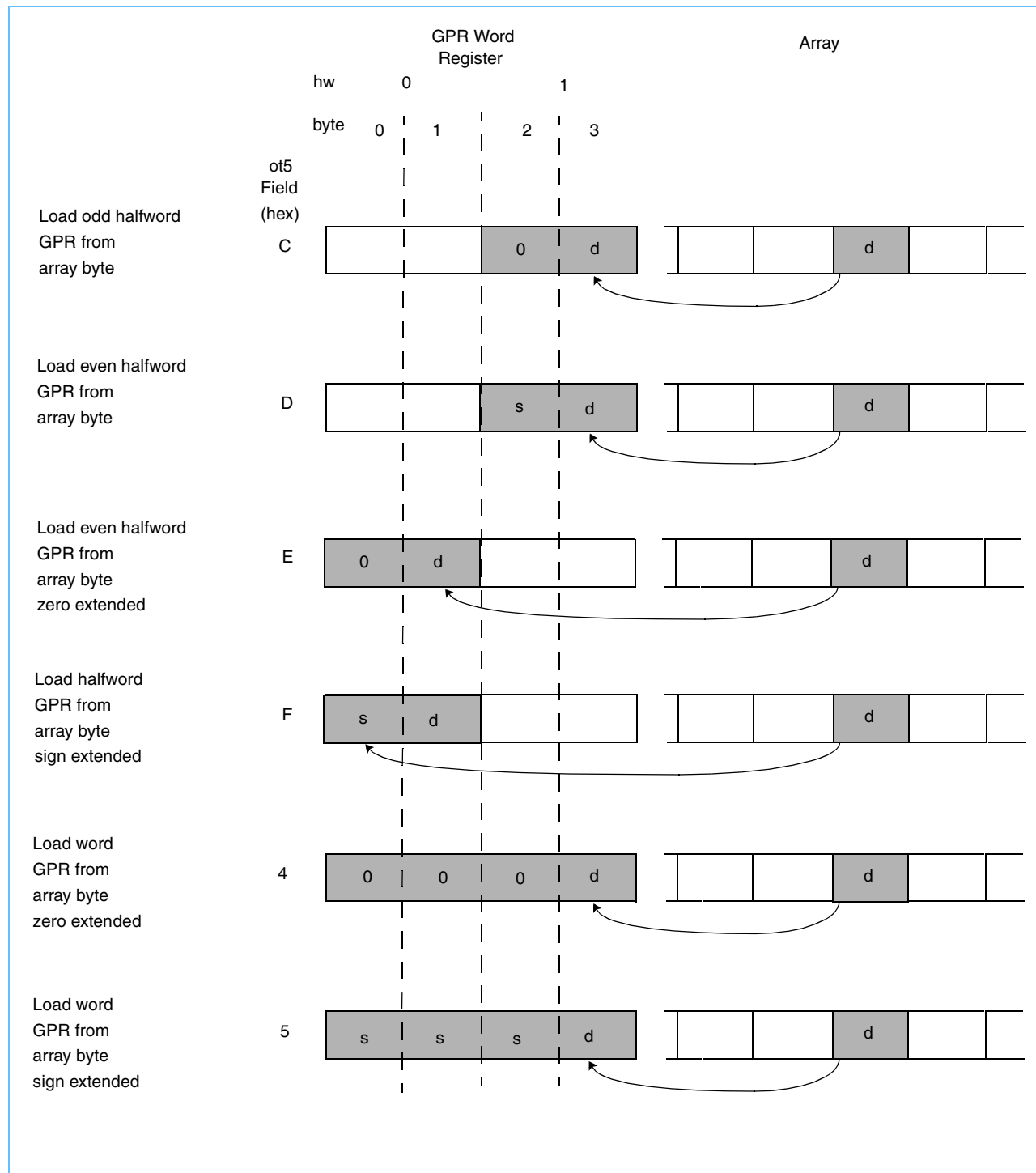
Figure 7-7. ot5 Field Definition: Loading GPR Halfword/Word from Array Byte
