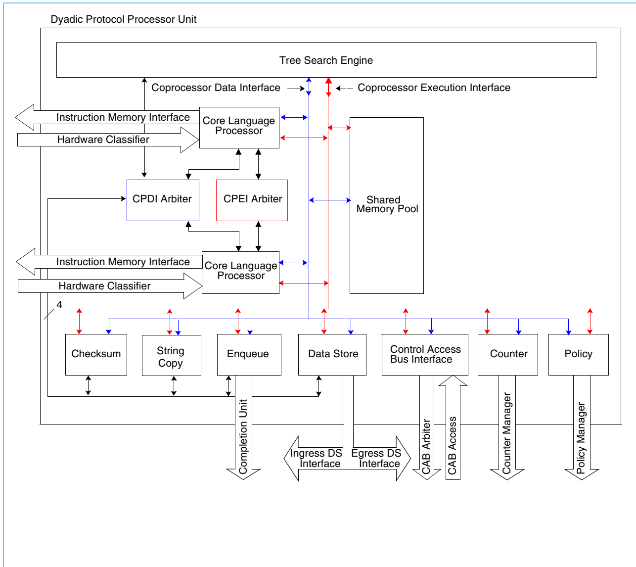
Figure 7-2. Dyadic Protocol Processor Unit Functional Blocks (NP4GS3A (R1.1))
