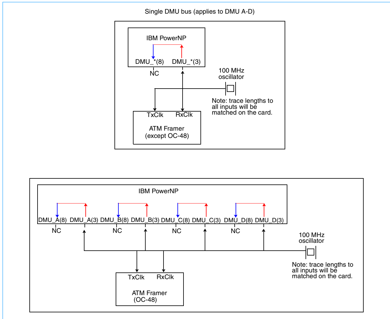
Figure 2-7. NP4GS3 DMU Bus Clock Connections (POS Overview)
