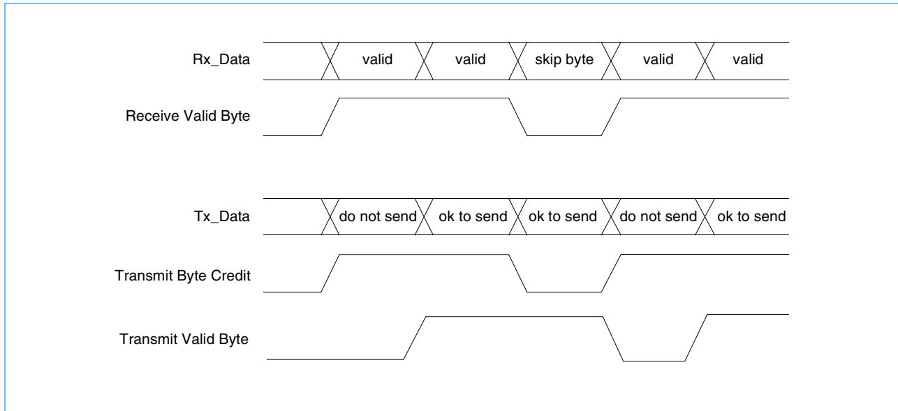
Figure 3-6. GMII POS Mode Timing Diagram
