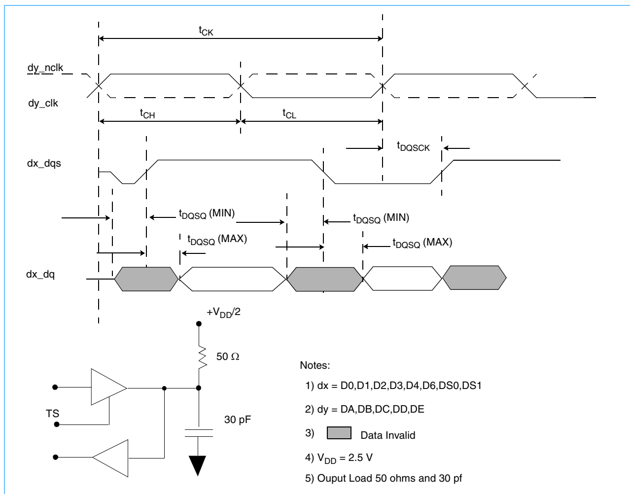
Figure 2-4. DDR Read Timing Diagram
