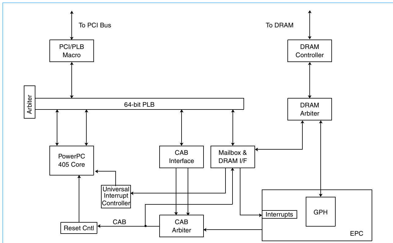
Figure 10-1. PowerPC Subsystem Block Diagram
