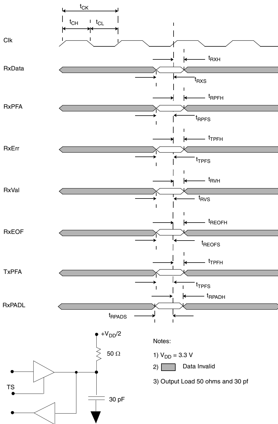
Figure 2-12. POS Receive Timing Diagram
