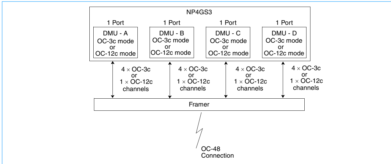
Figure 3-8. OC-48 Configuration
