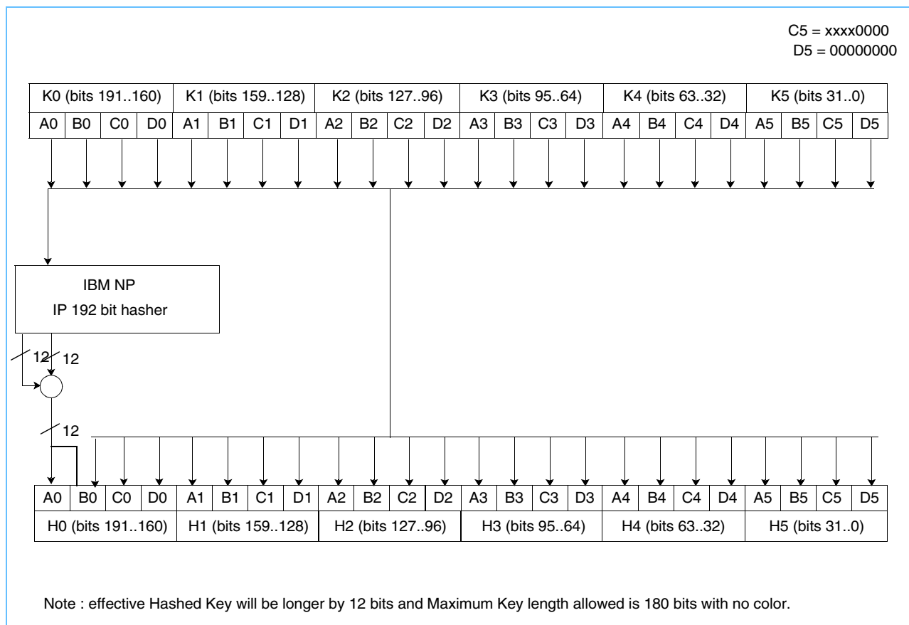
Figure 8-16. 12-bit Hash Function
