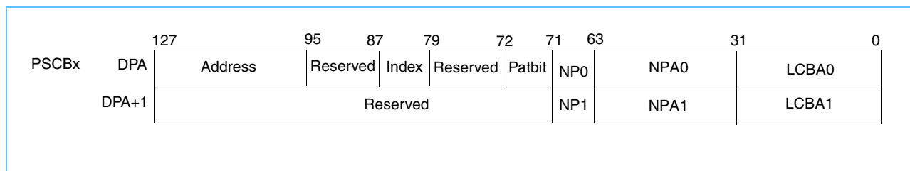
Figure 8-8. Shared Memory Pool with PSCB subfields
