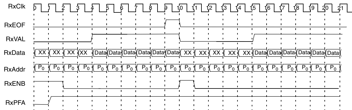
Figure 3-12. Receive POS8 Interface Timing for 8-bit Data Bus (OC-12c)
