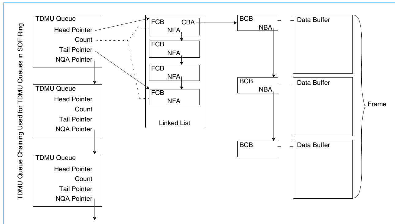
Figure 4-3. Ingress EDS Logical Structure
