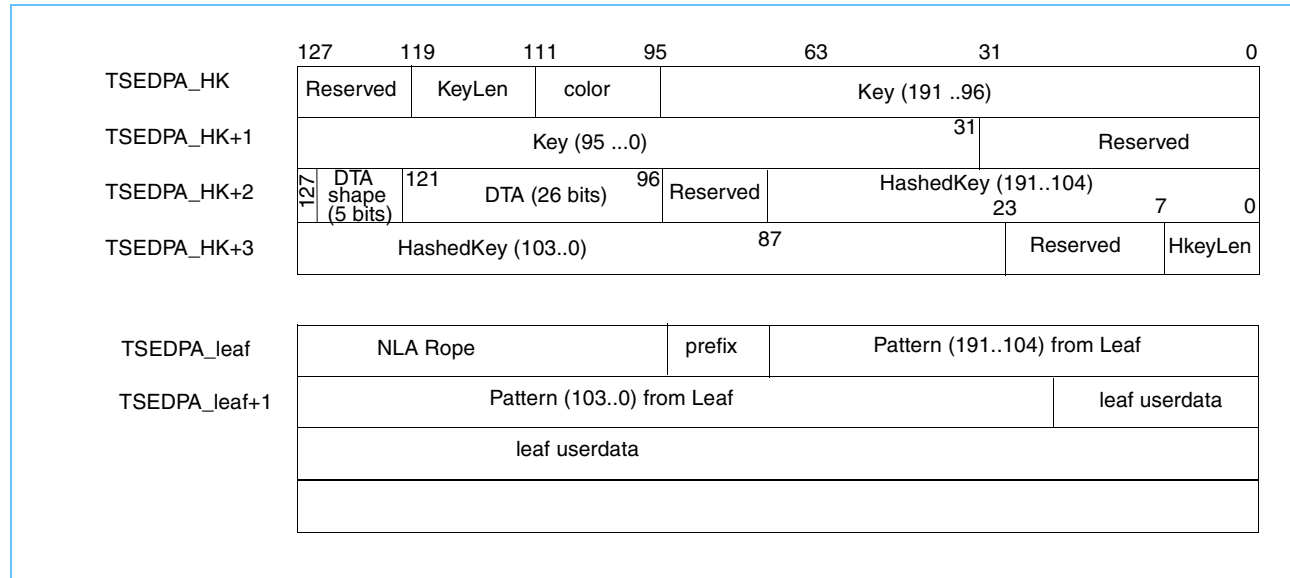
Figure 8-7. Shared Memory Pool with DISTPOS_GDH Command Subfields
