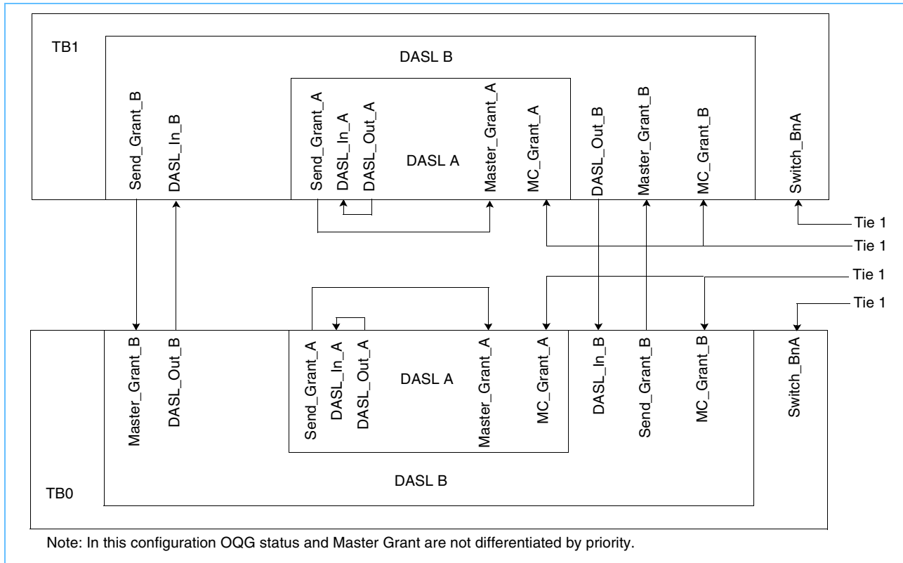
Figure 5-5. External Wrap Mode (Two NP4GS3 interconnected)
