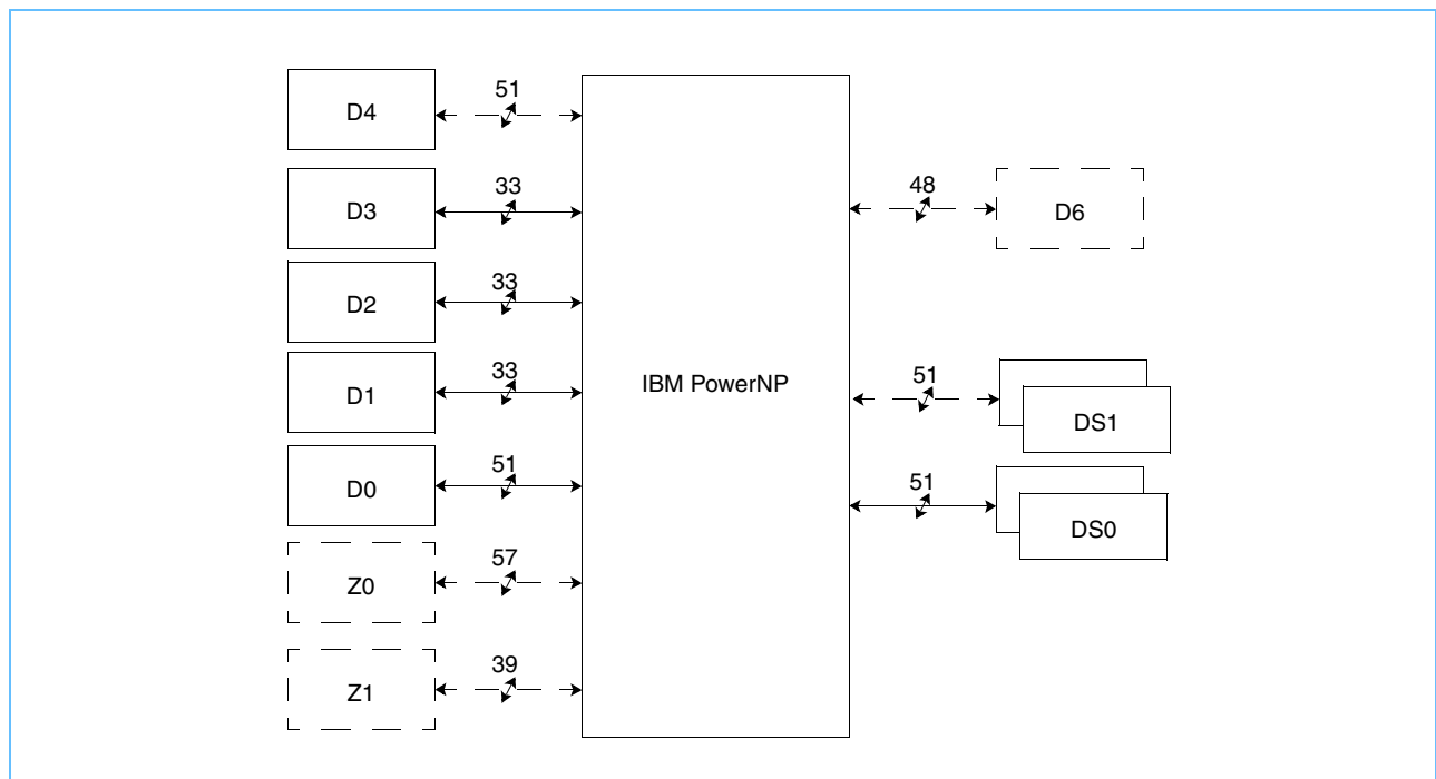
Figure 13-1. NP4GS3 Memory Subsystems
