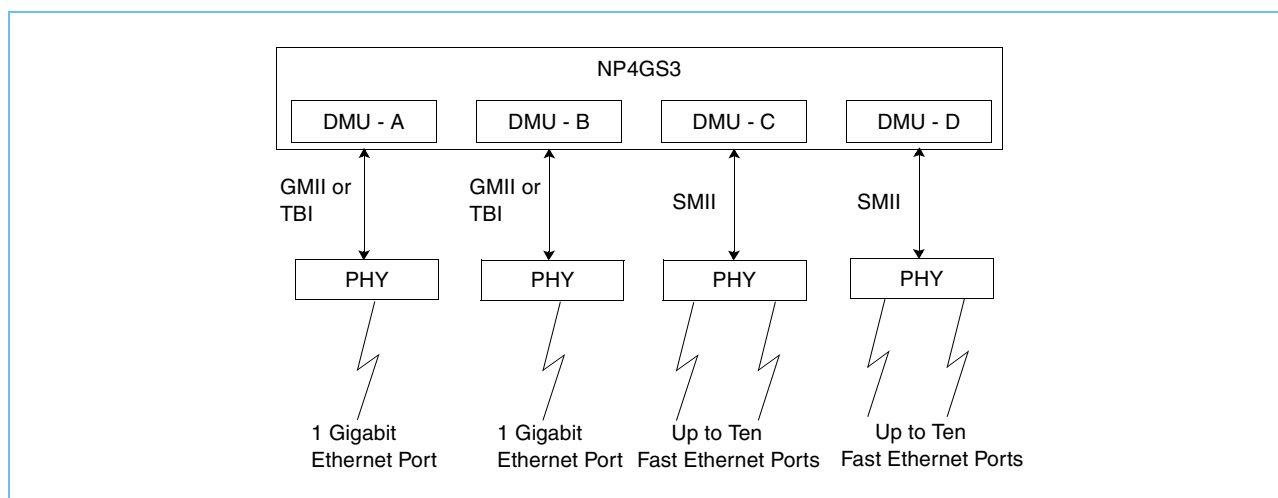
Figure 3-2. Ethernet Mode
