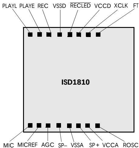
Figure 10: ISD1810 Bonding Physical Layout (Unpackaged Die)
