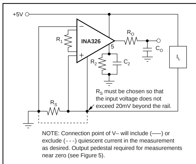
FIGURE 7. Low-Side Shunt Measurement of Current Load.
