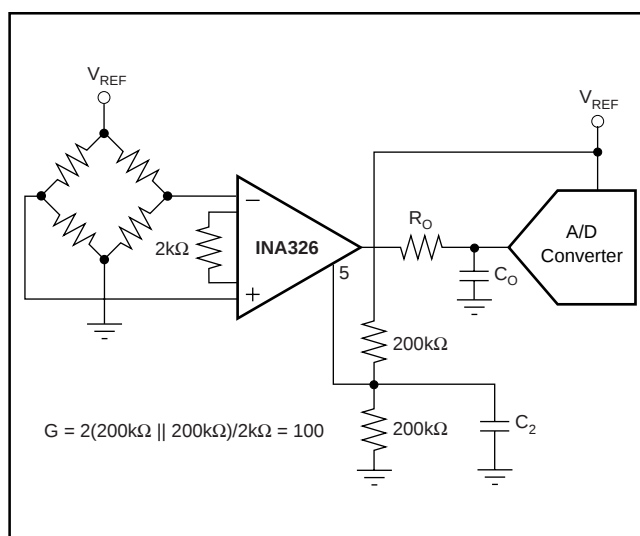
FIGURE 8. Output Referenced to V_{REF}/2 .
