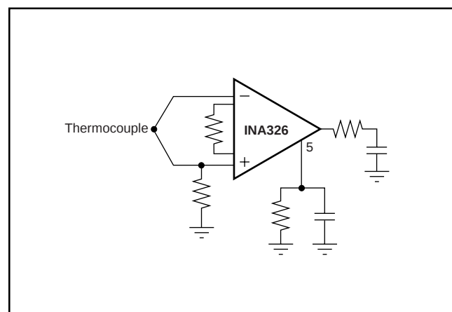
FIGURE 3. Providing Input Bias Current Return Path.
