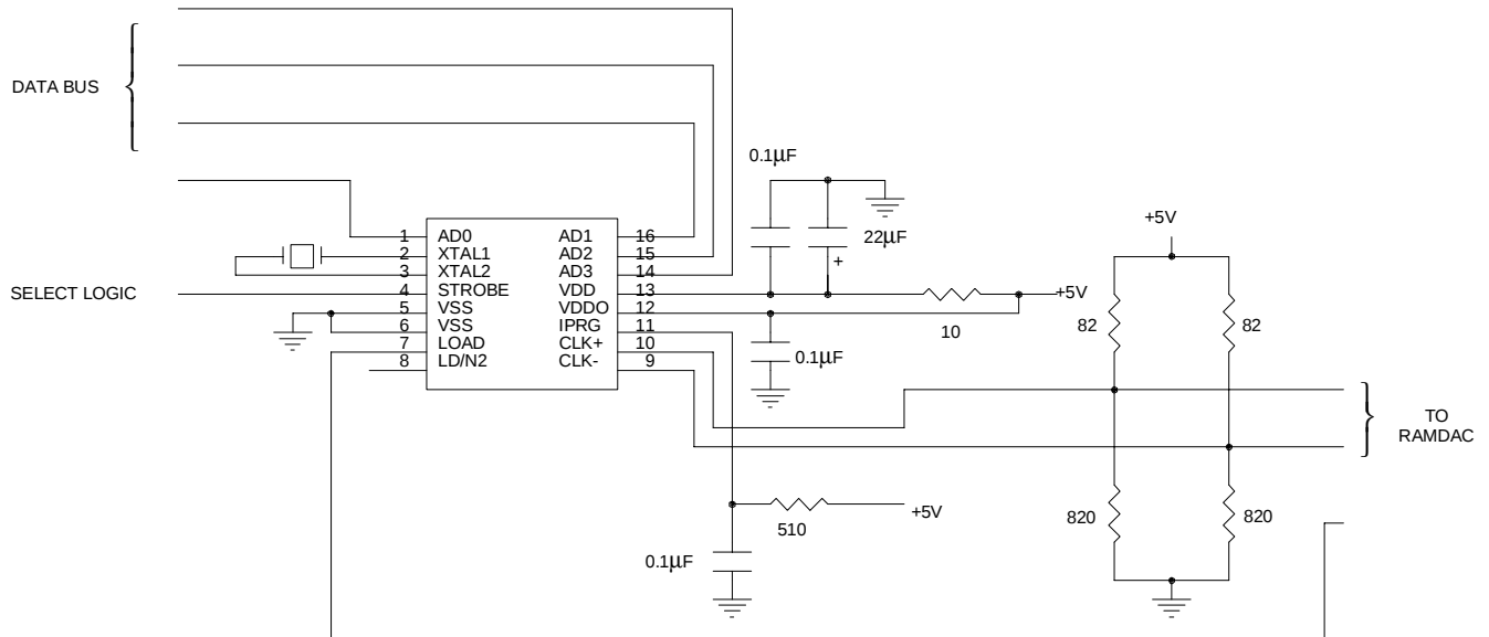
ICS1562A-001 Typical Interface
