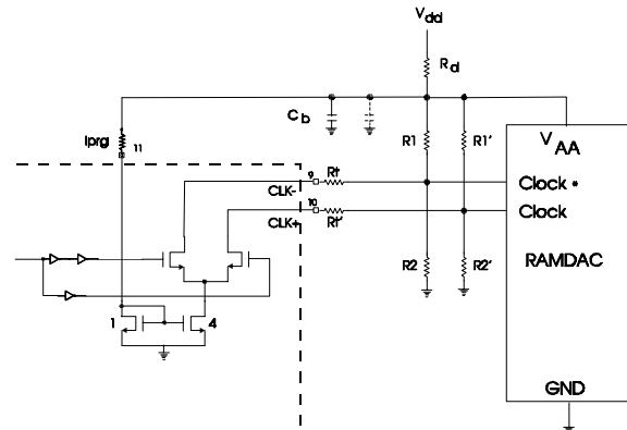
ICS1562A Output Circuitry
