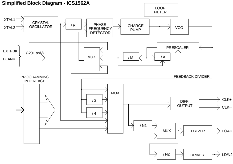
Simplified Block Diagram - ICS1562A
