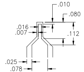
50Ω lead transition
