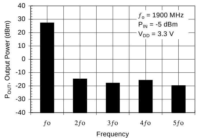
Figure 5. Harmonics
