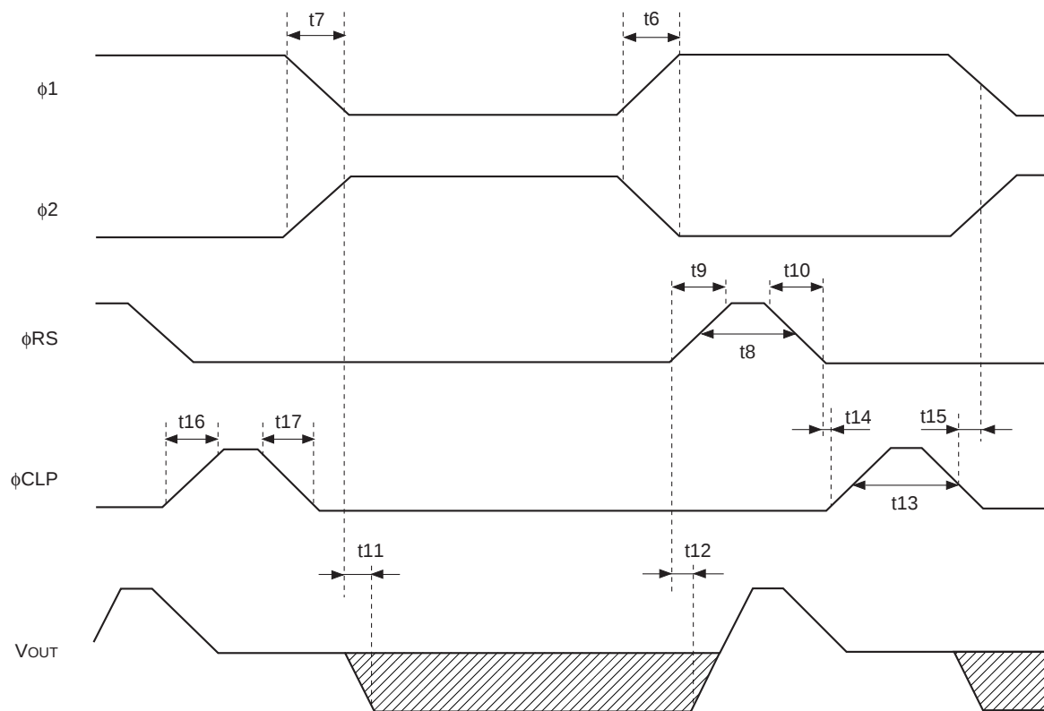
Clock Timing Chart 3
