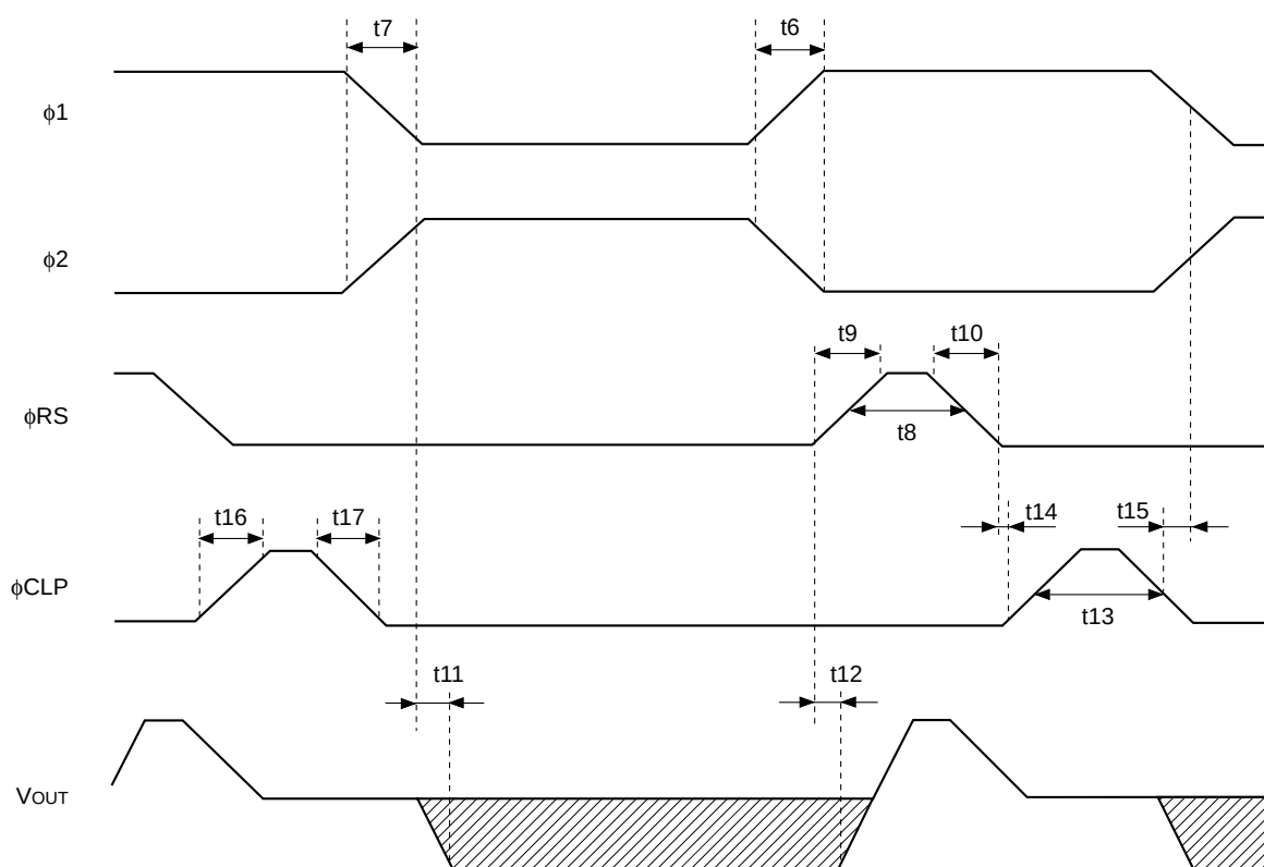
Clock Timing Chart 3
