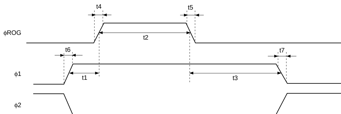
Clock Timing Chart 2
