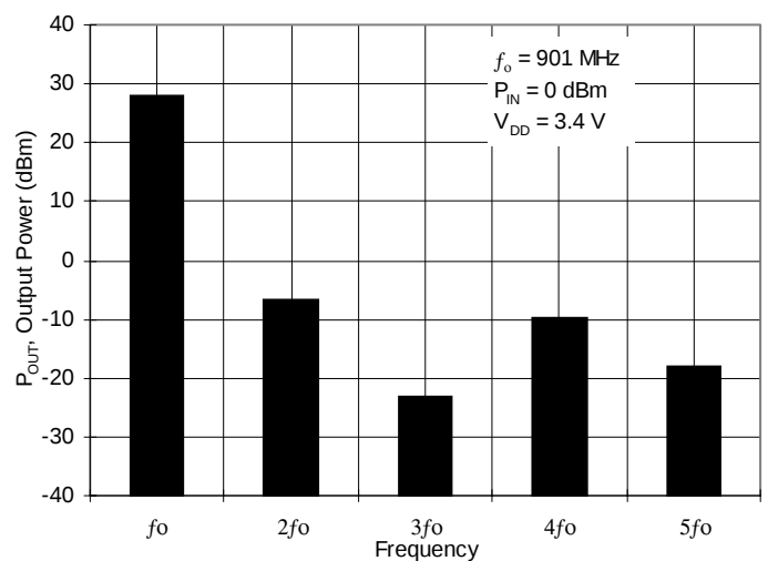
Figure 5. Harmonics
