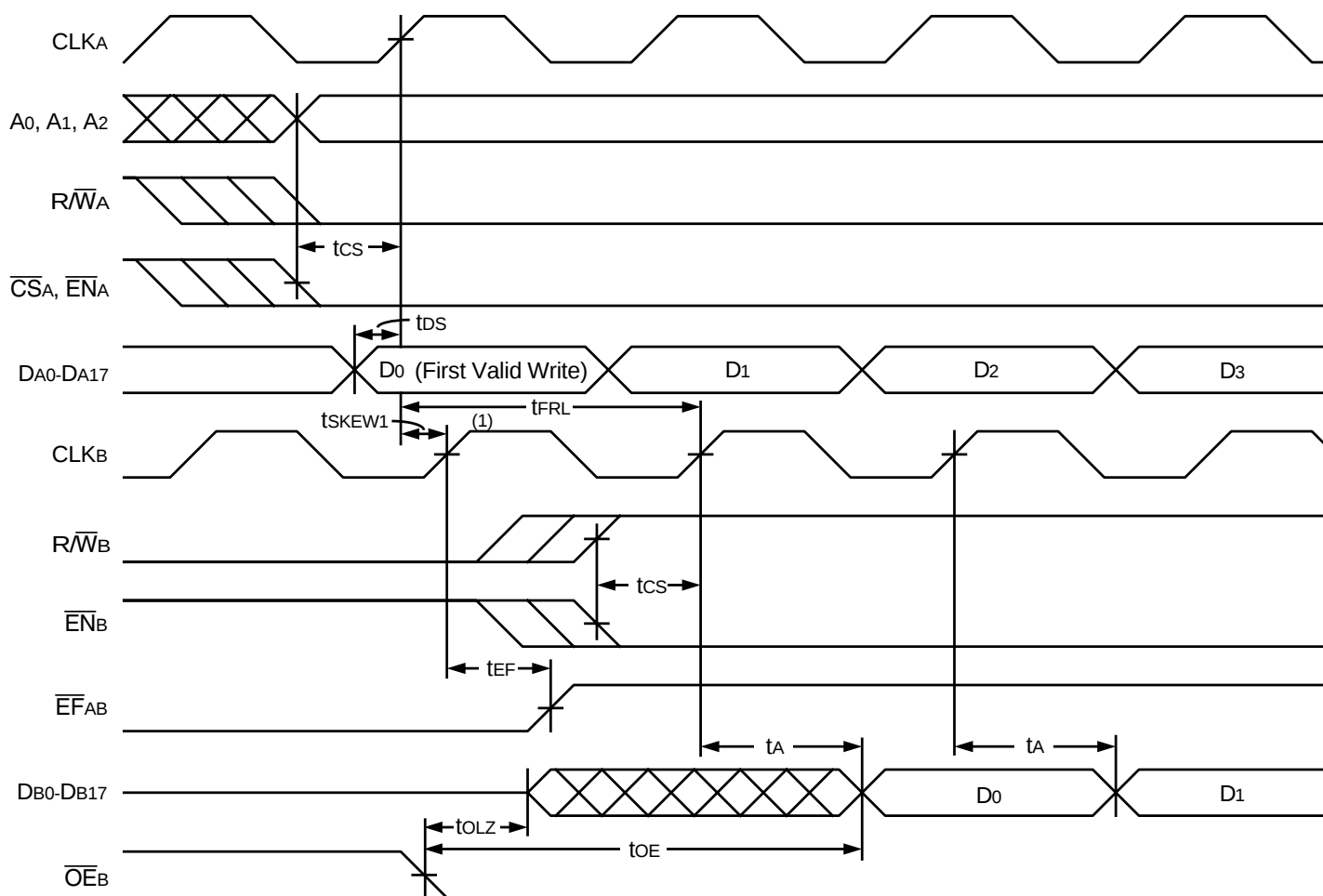
Figure 7. Port B (A→B) Read Timing
