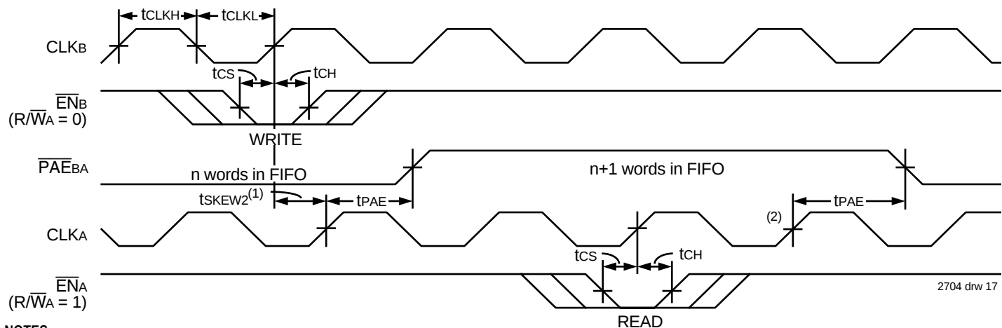
Figure 13. A→B Programmable Almost-Full Flag Timing
