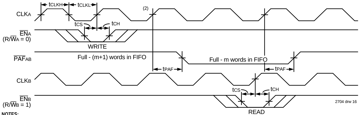
Figure 12. A→B Programmable Almost-Empty Flag Timing
