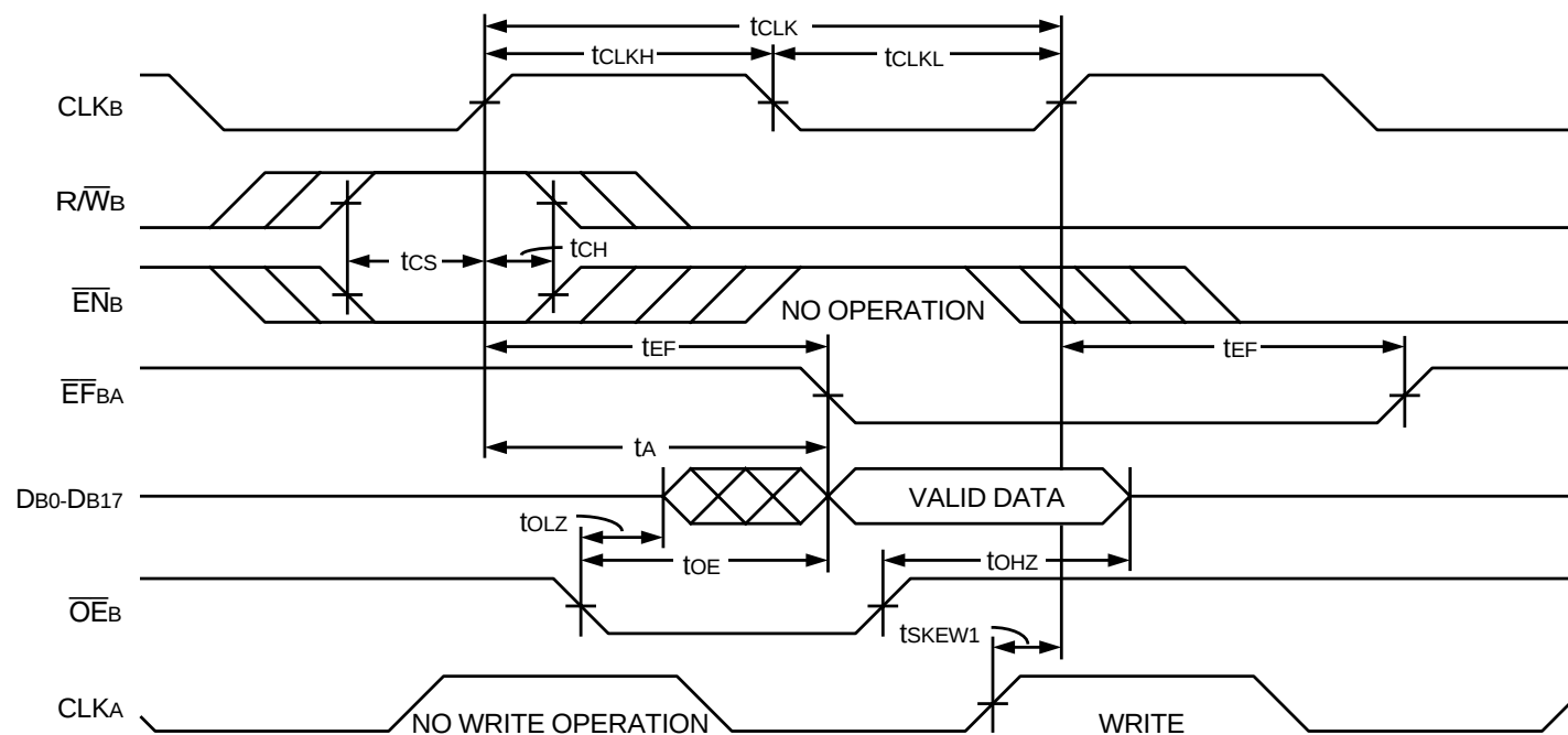
Figure 7. Port B (A→B) Read Timing
