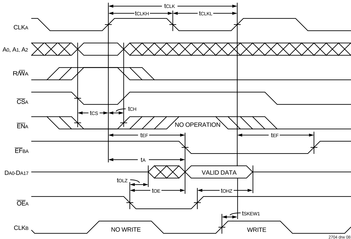
Figure 5. Port A (B→A) Read Timing
