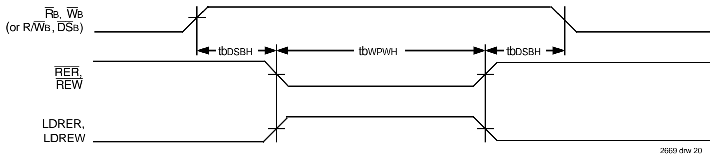
Figure 18. Port B Reread and Rewrite Timing for Intelligent Retransmit
