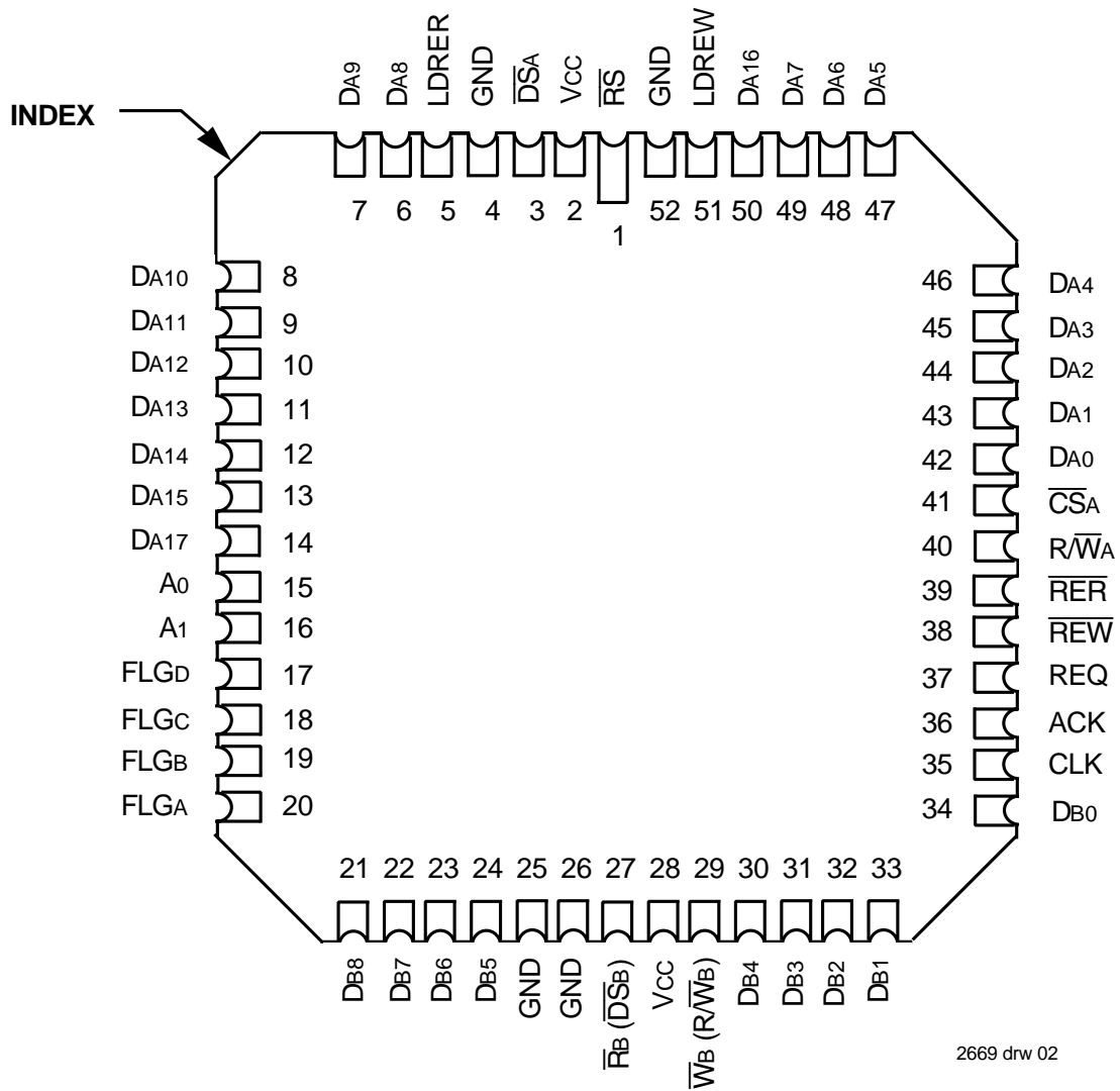
PLCC (J52-1, order code: J) TOP VIEW
